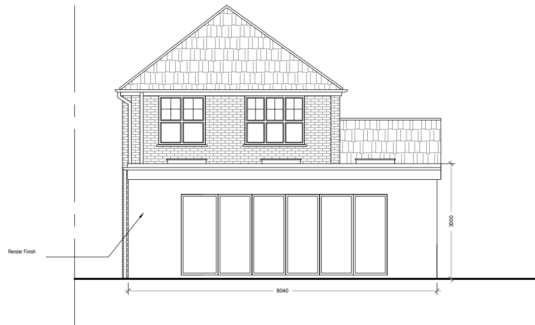
Rear Elevation
