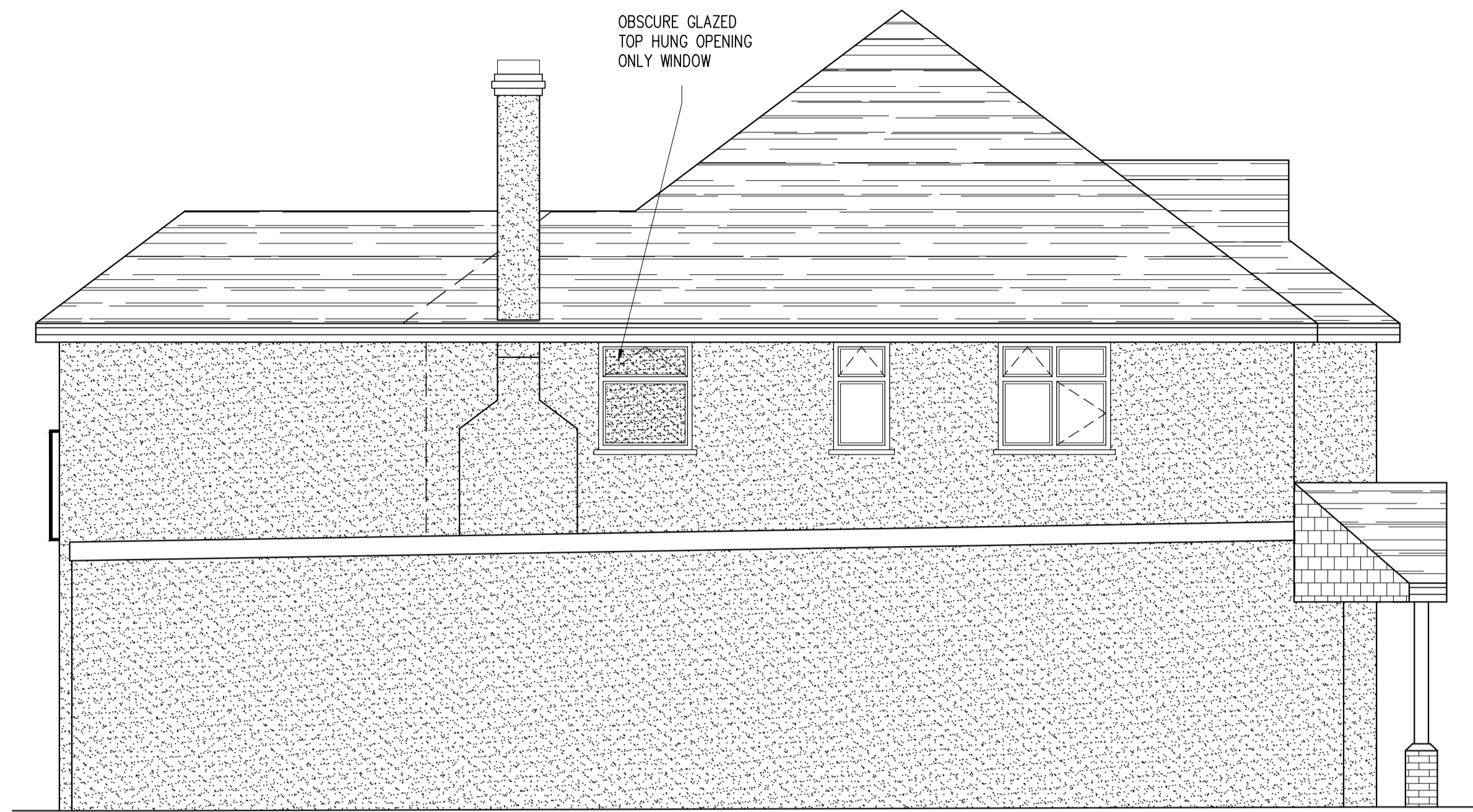
PROPOSED SIDE ELEVATION A SCALE 1:50
