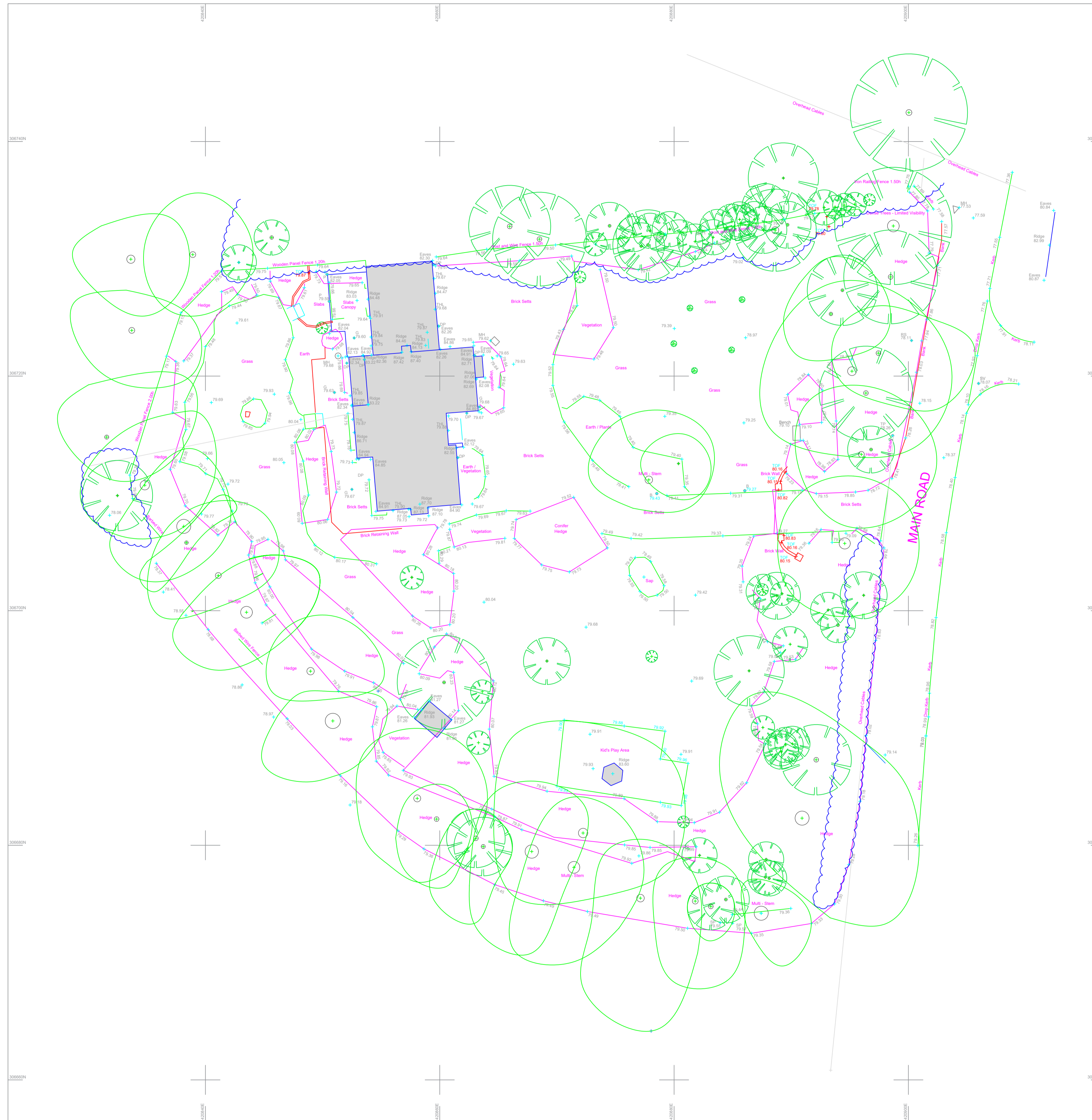
Existing Site Plan with Topography [1:200]
