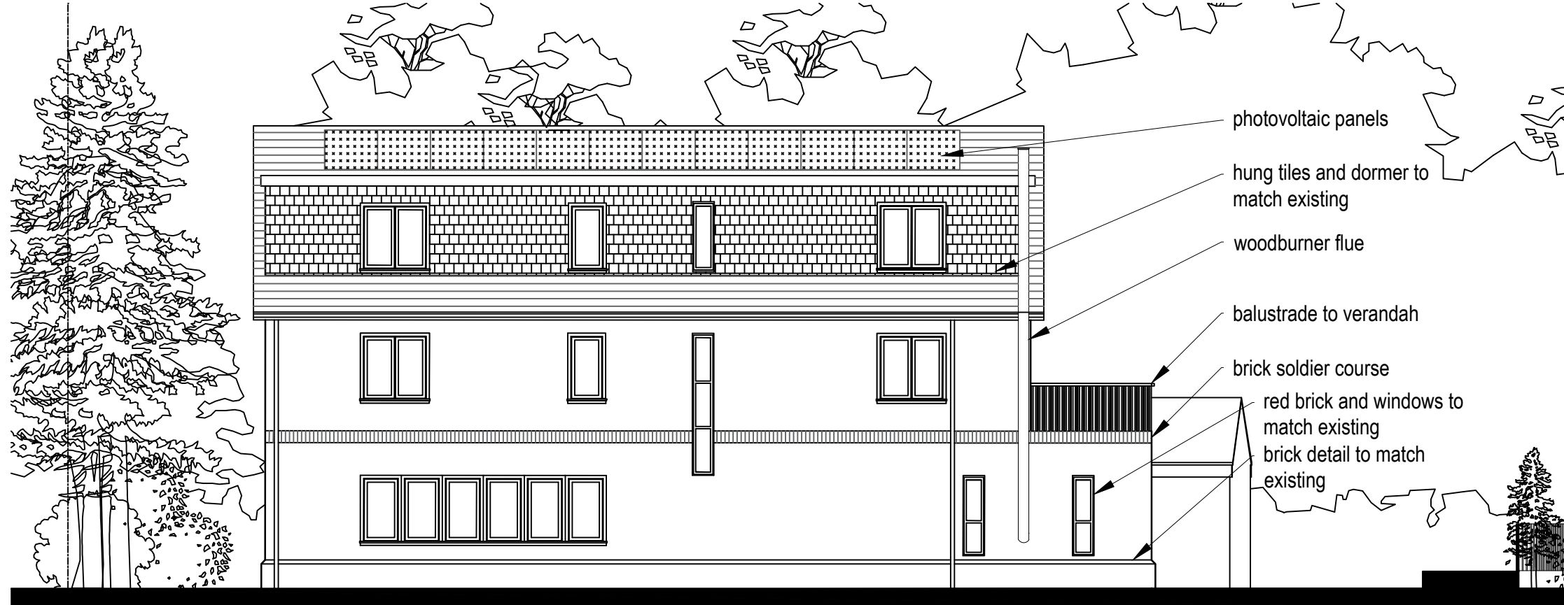
South elevation
