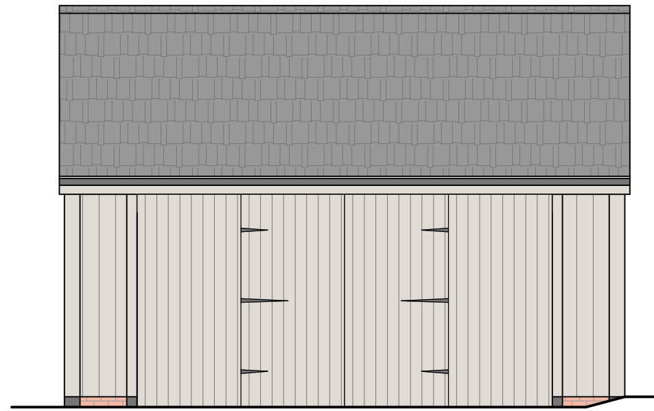
SOUTH ELEVATION
