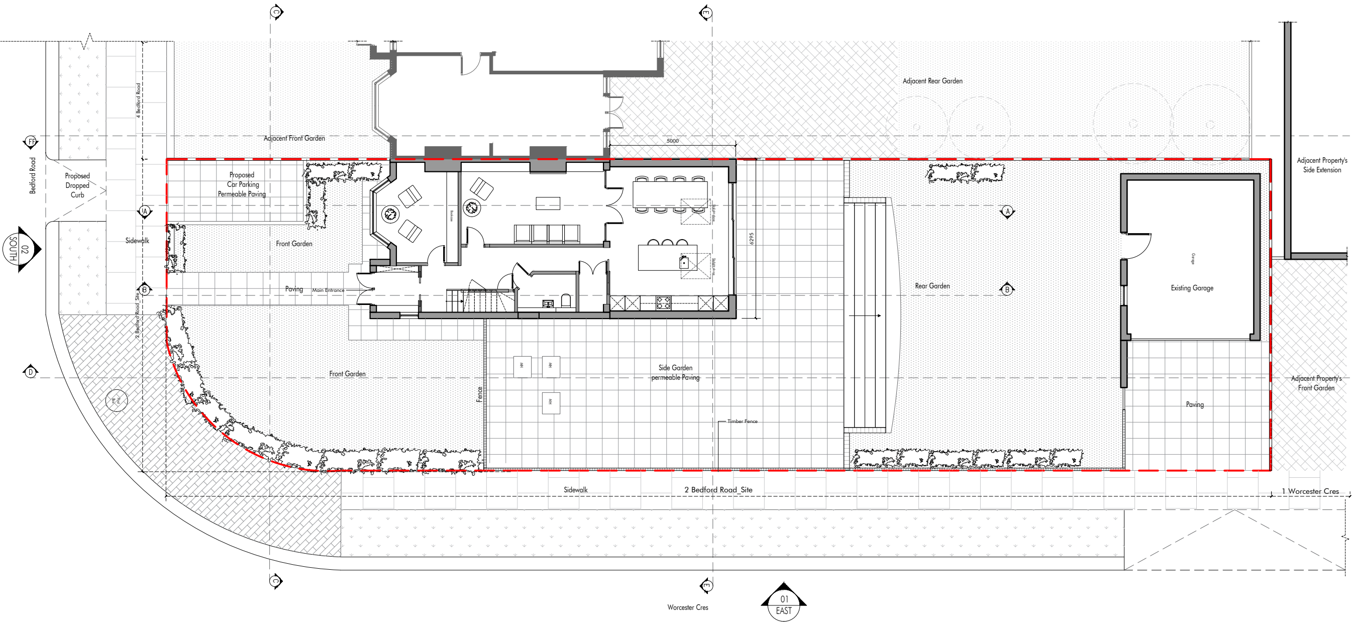
Proposed Site Plan Scale 1:150
