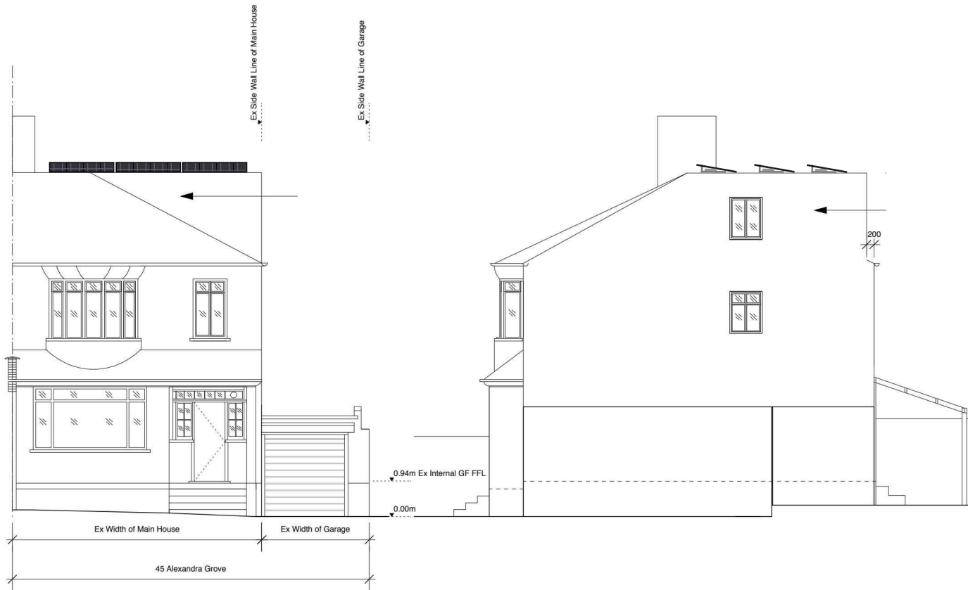
Proposed Side Elevation v1.0 25 May 2022
