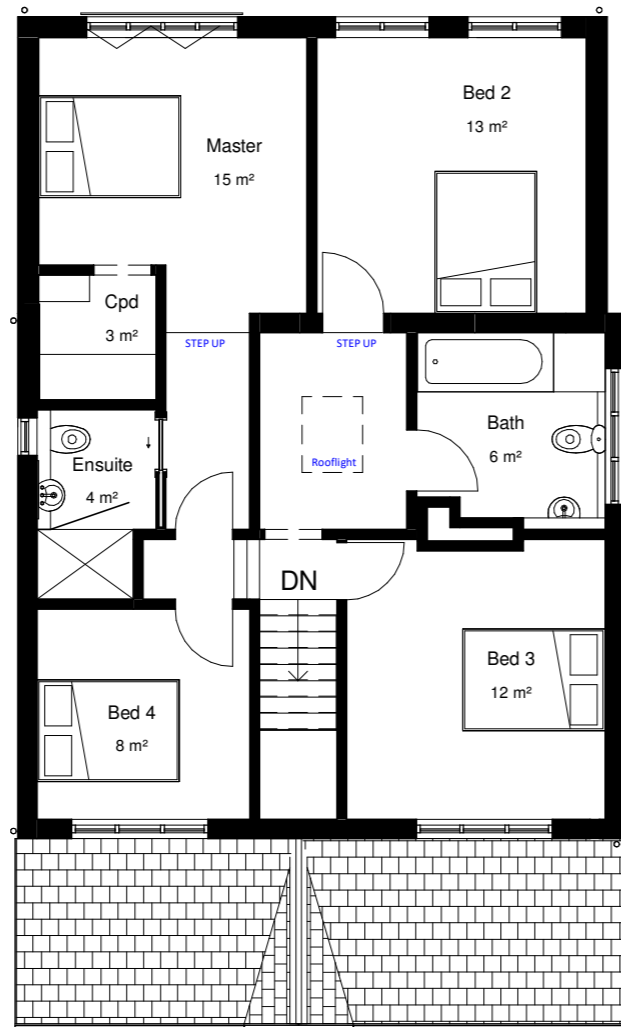
GA First Floor Plan As Proposed 1 : 100
