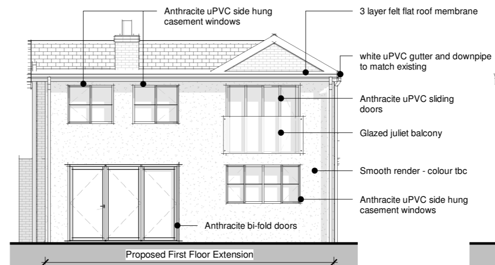
North Elevation As Proposed 1 : 100
