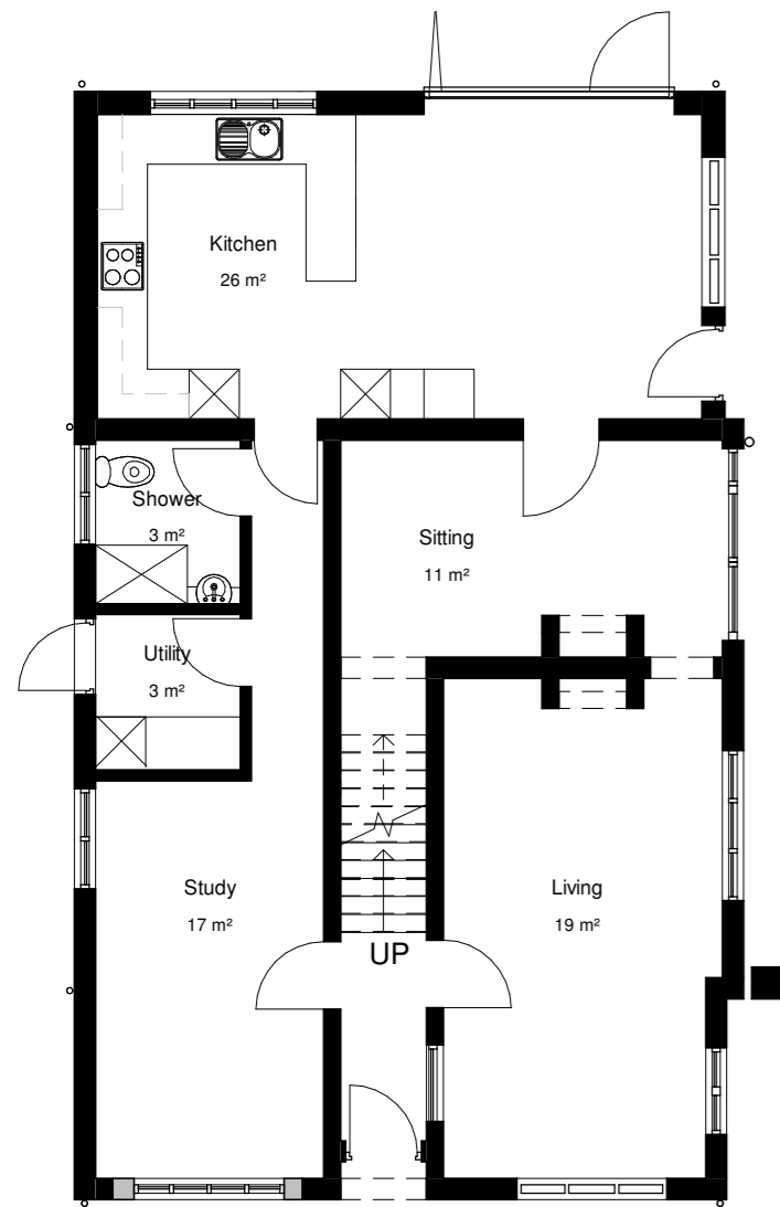
GA Ground Floor Plan As Proposed 1 : 100
