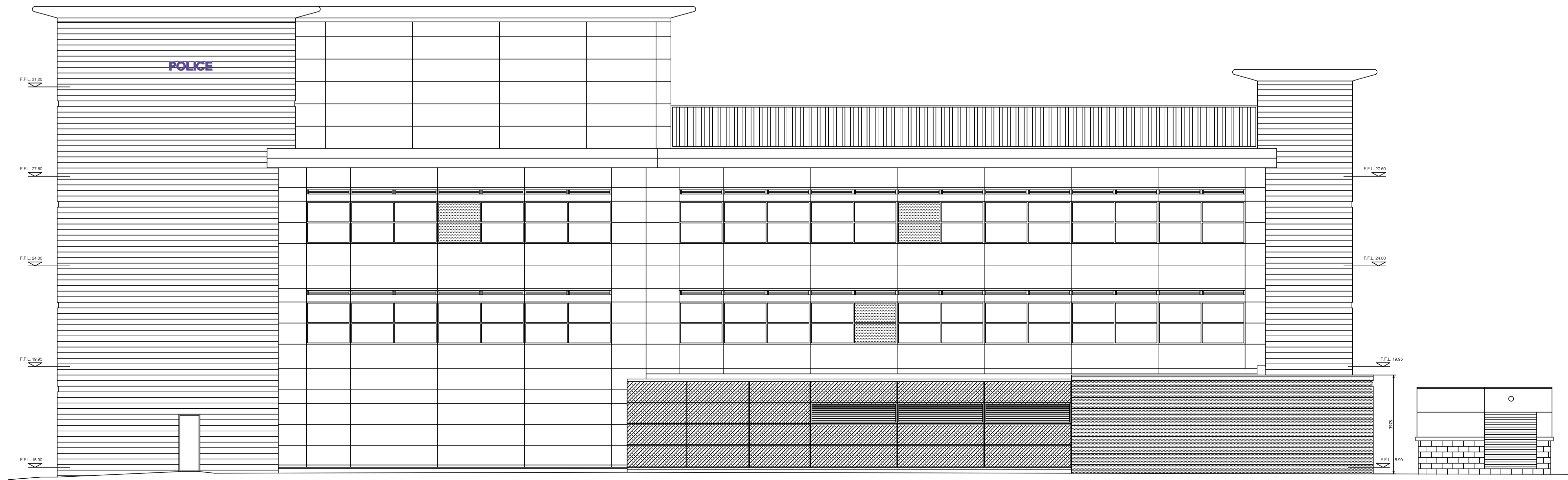
EXISTING WEST (Helen Street) ELEVATION Scale 1:100
