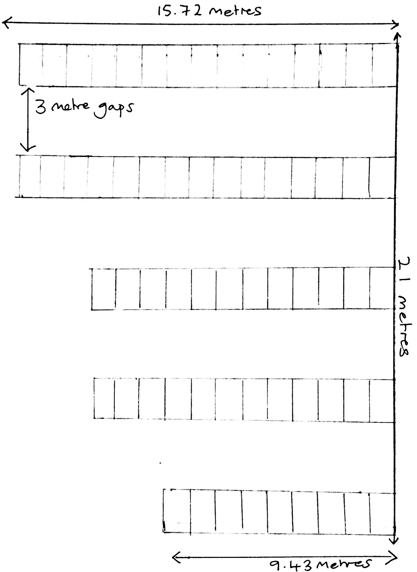
Crandon Farm Solar Panel plan. 64 panels - 1765 x 1048 mm each
