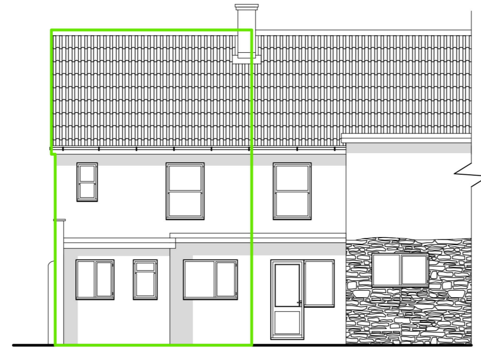
REAR ELEVATION
