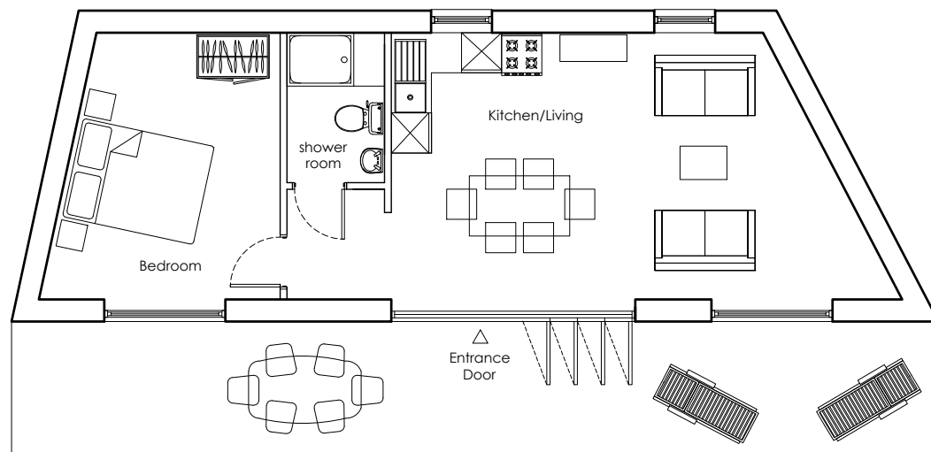
Floor Plan
