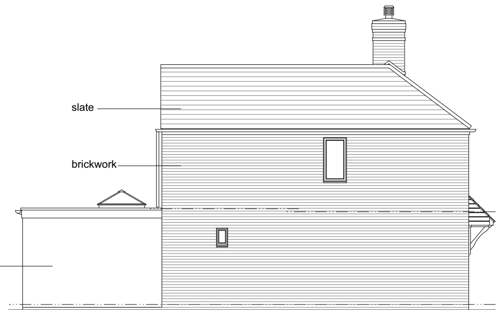
Existing side (west) elevation
