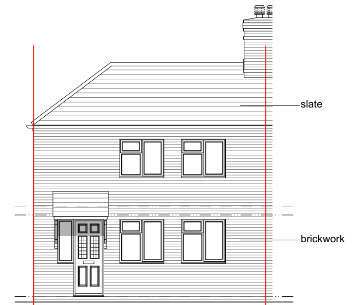
Existing front (south) elevation
