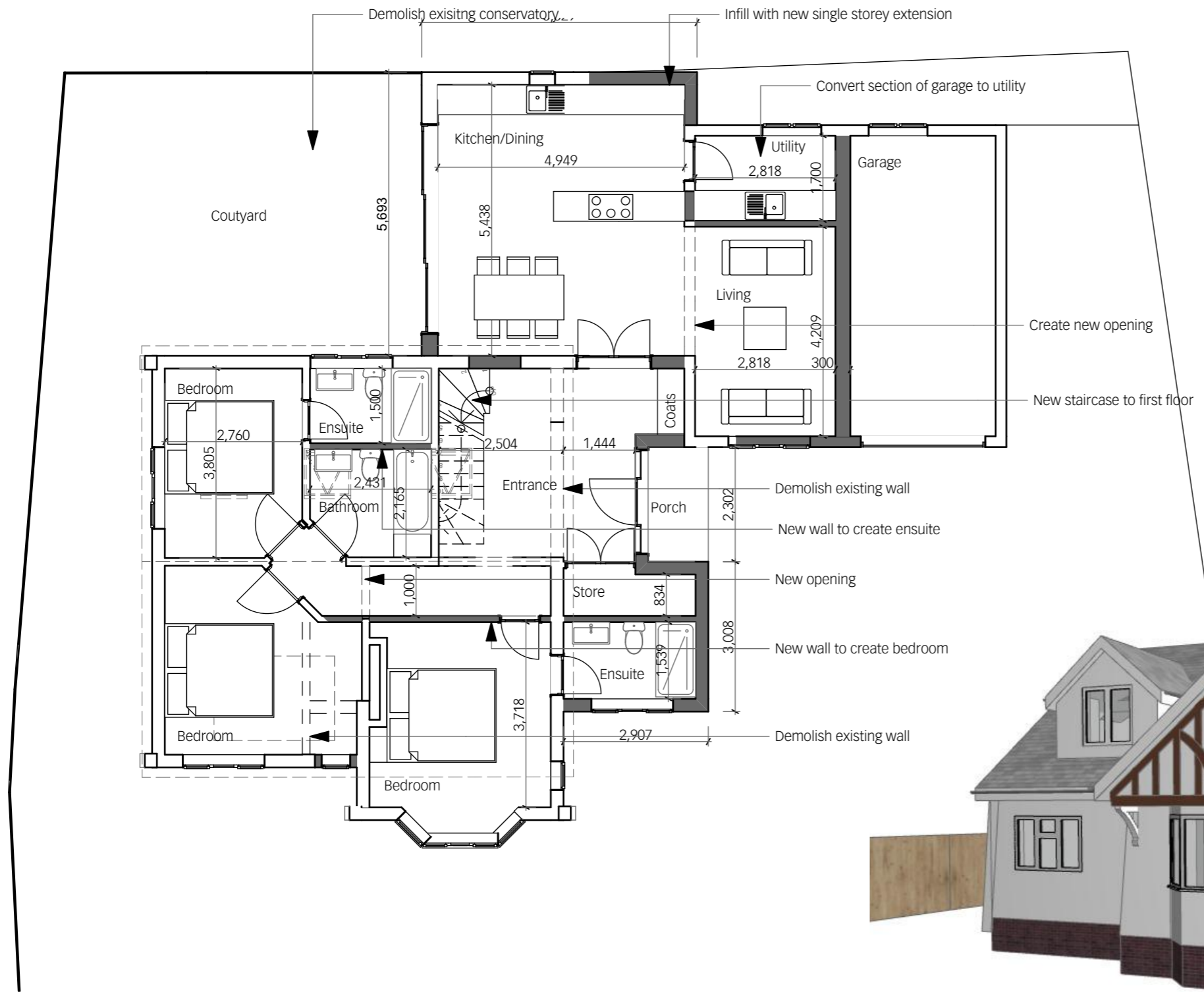
1 Ground Floor Plan 1:100
