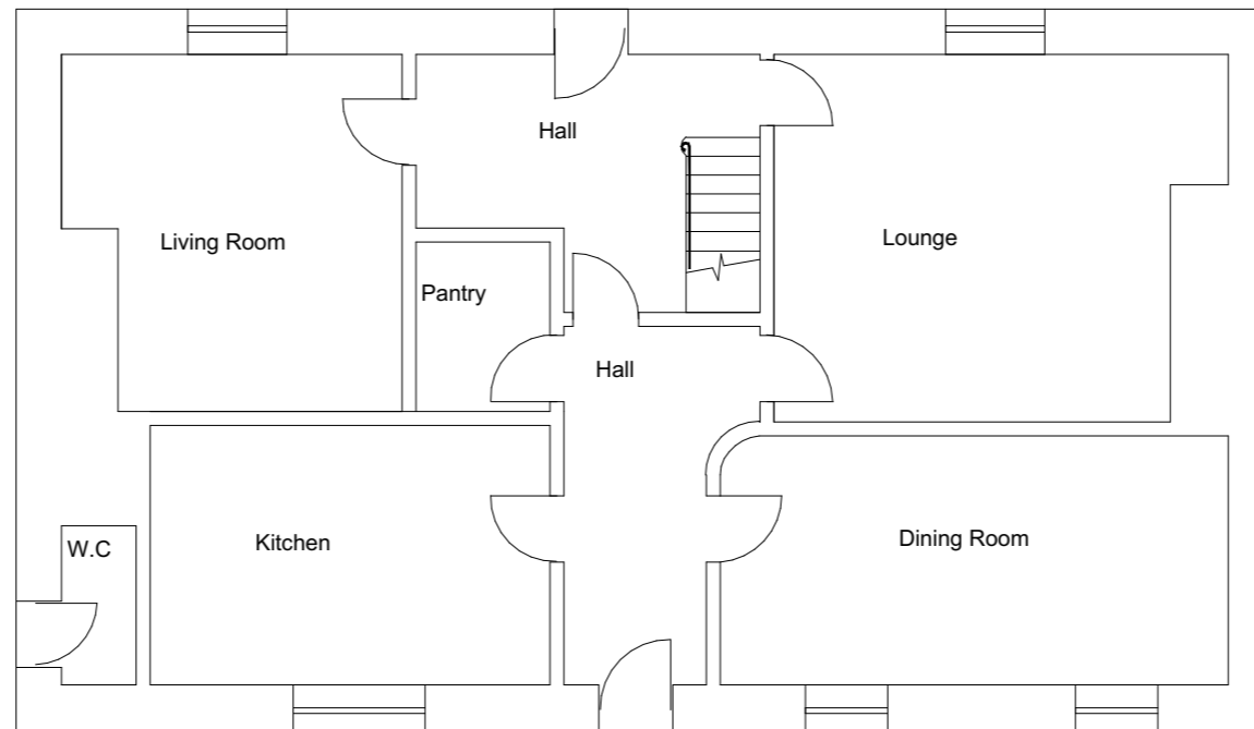
Original House Ground Floor Plan 1:100 @ A3
