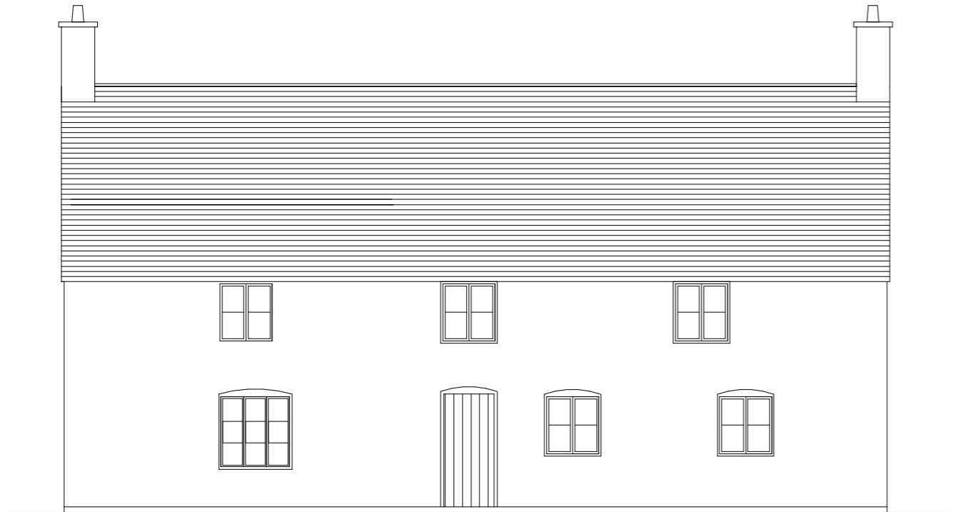
Rear Elevation 1:100 @ A3
