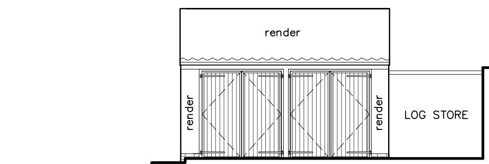
GARAGE FRONT ELEVATION
