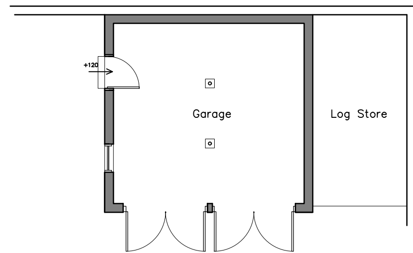
GARAGE PLAN
