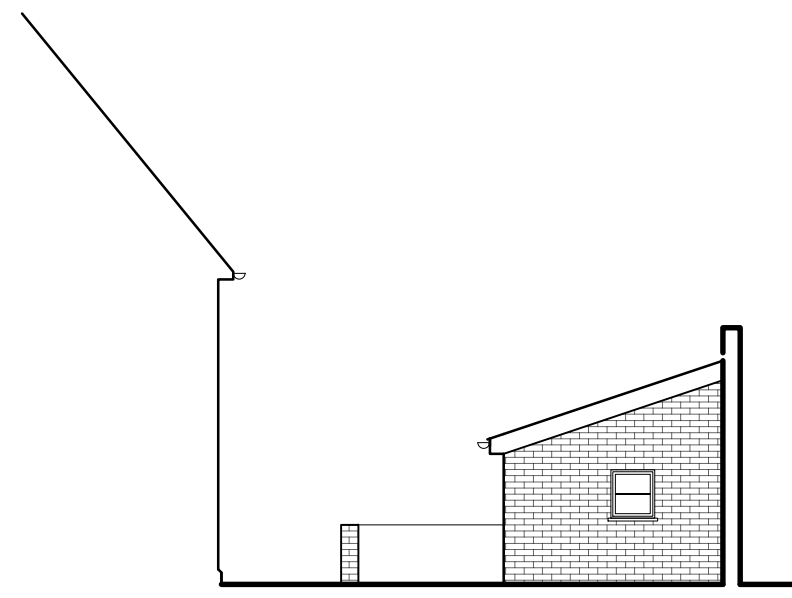
OUTBUILDING SIDE ELEVATION
