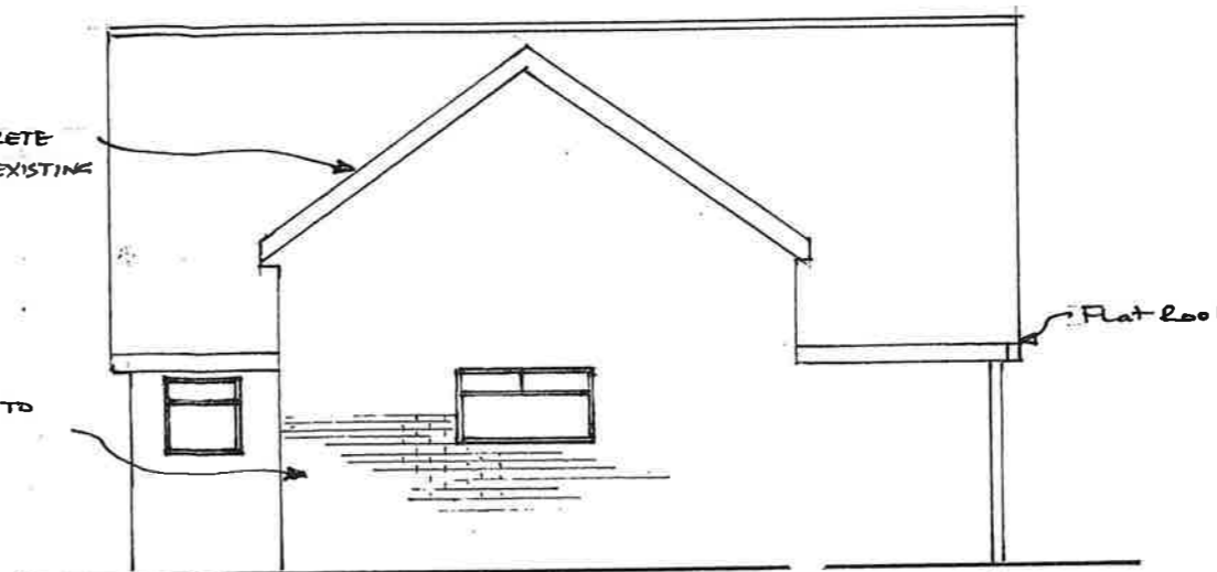
NORTH ELEVATION. 1:100
