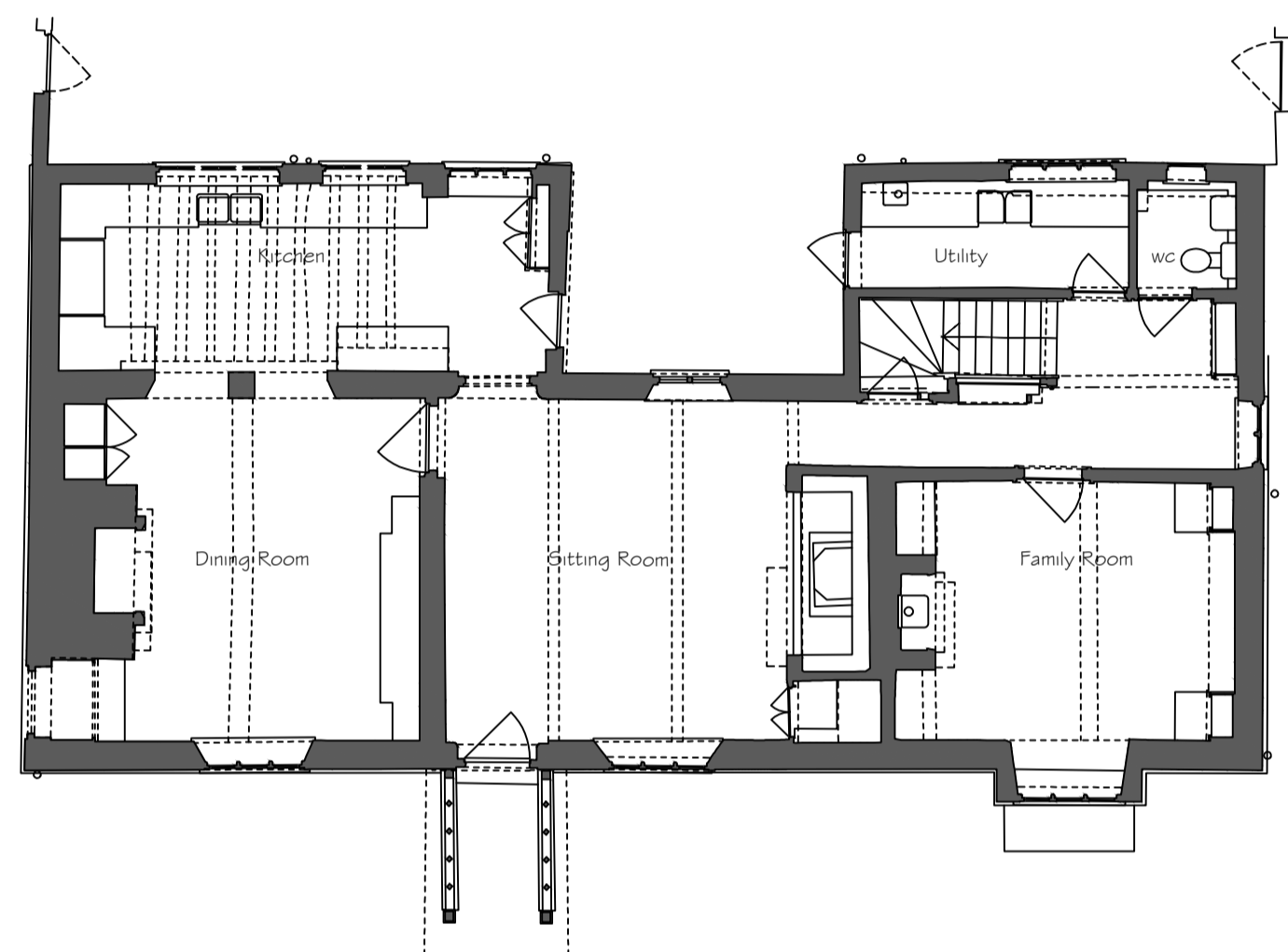
2 Ground Floor 1 : 100
