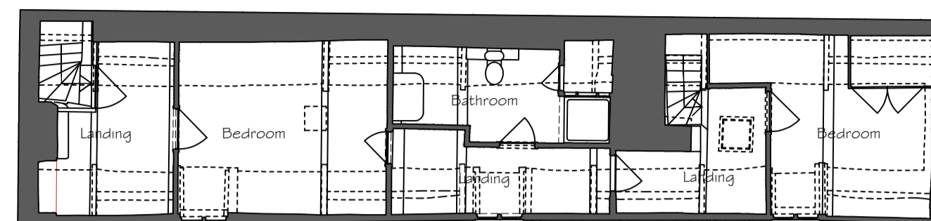
4 Second Floor 1 : 100
