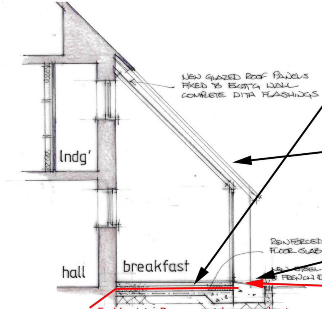
Section C-C 1:50
