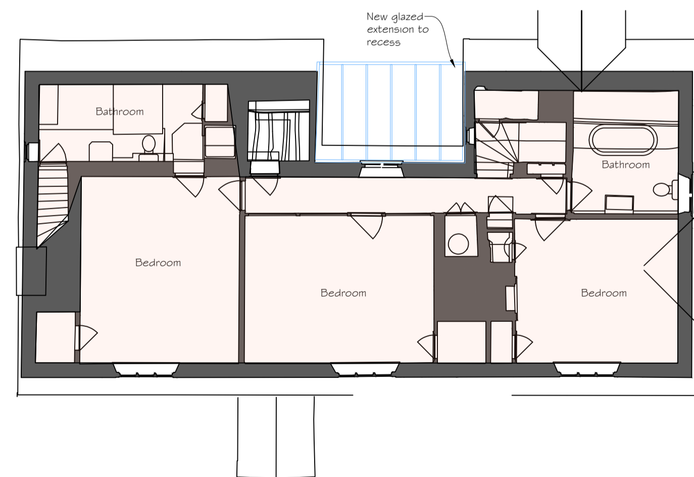
3 First Floor 1 : 100
