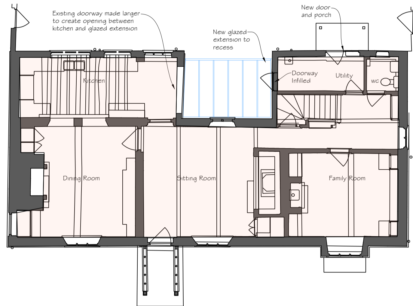
2 Ground Floor 1 : 100
