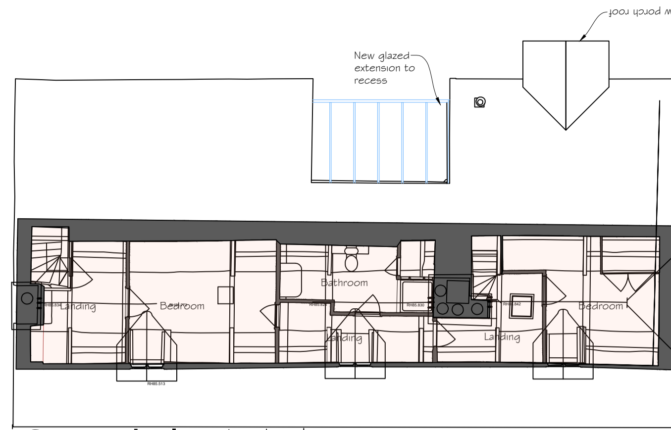
4 Second Floor 1 : 100
