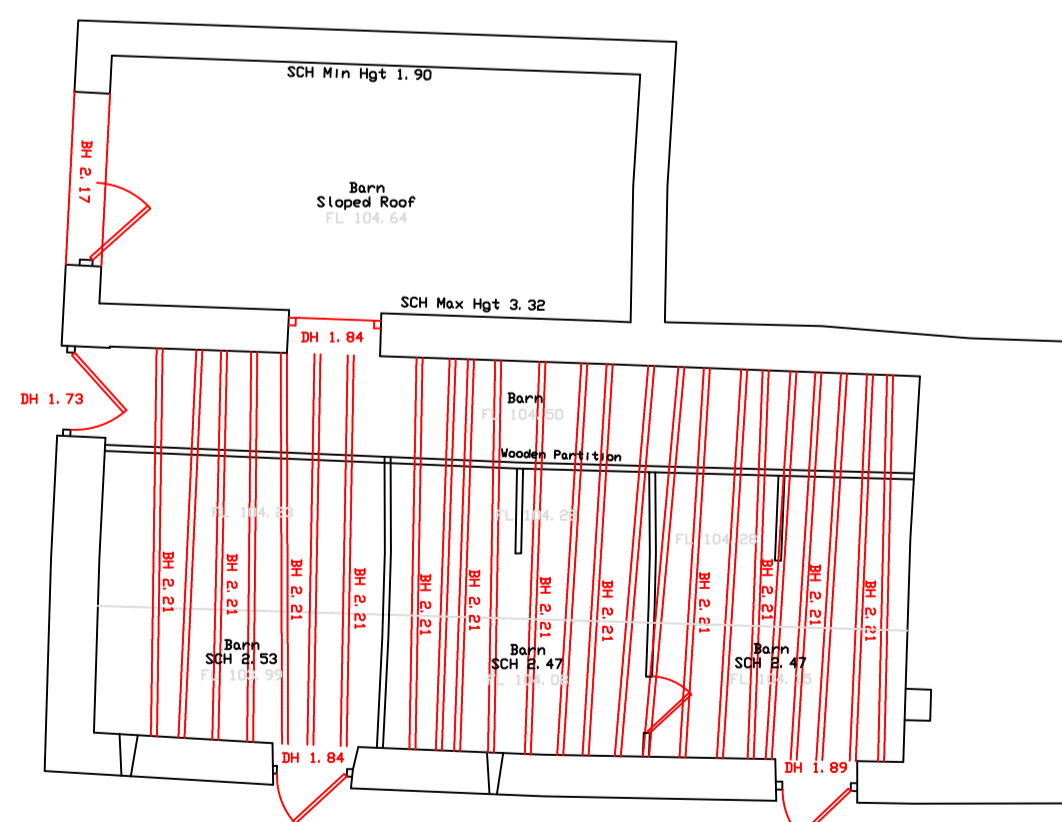
Barn 2 Ground Floor Plan
