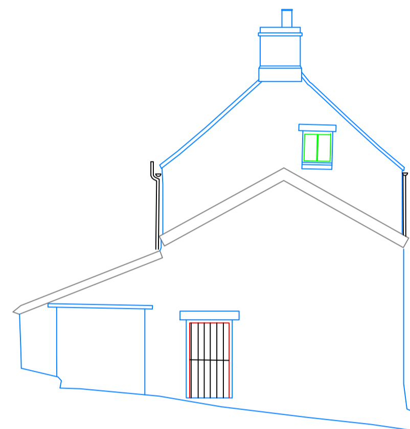
Barn 2 West Elevation
