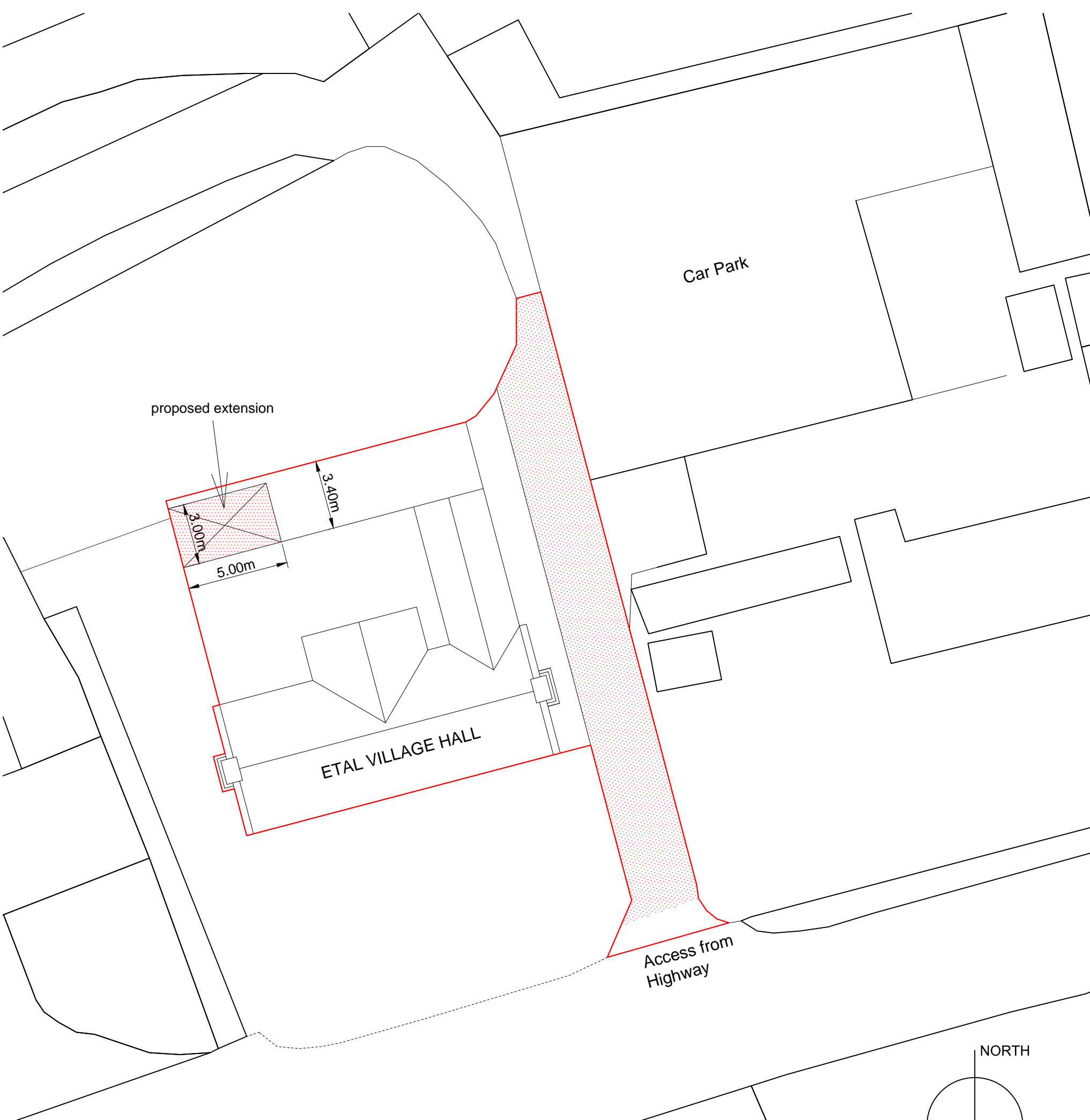
SITE LAYOUT 1:200 scale @A3 size
