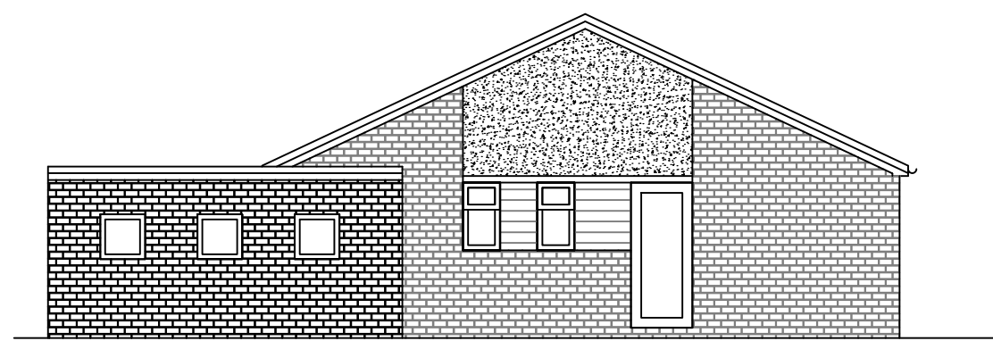
EXISTING GABLE ELEVATION
