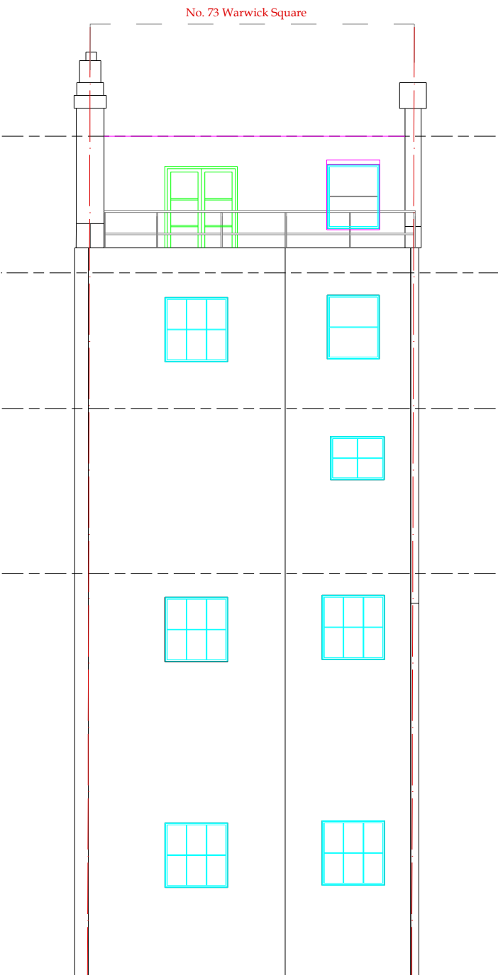
Rear Elevation
