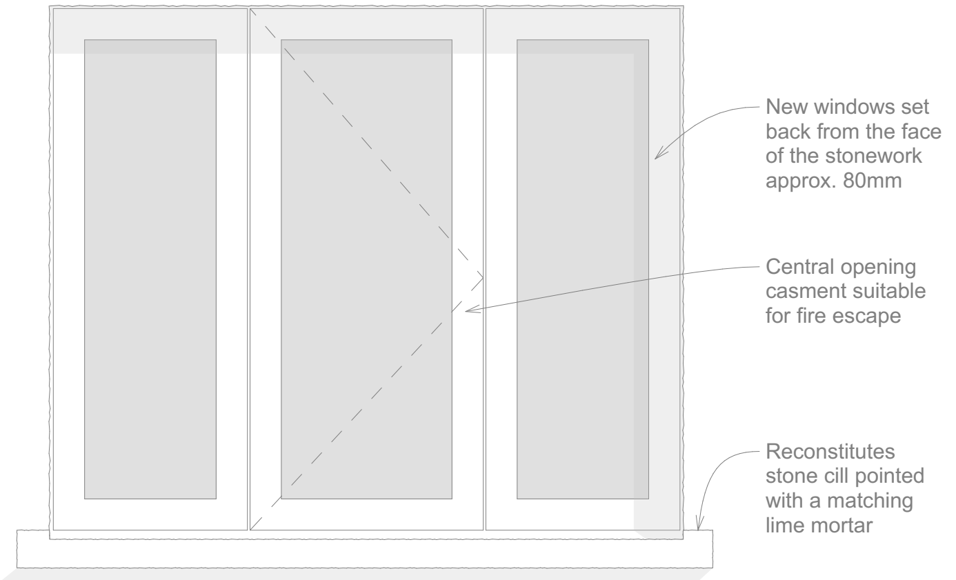
EXTERNAL ELEVATION @ 1:10
