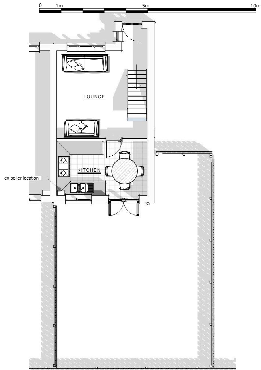
E 1 :: EXISTING GROUND FLOOR PLAN scale: 1:100
