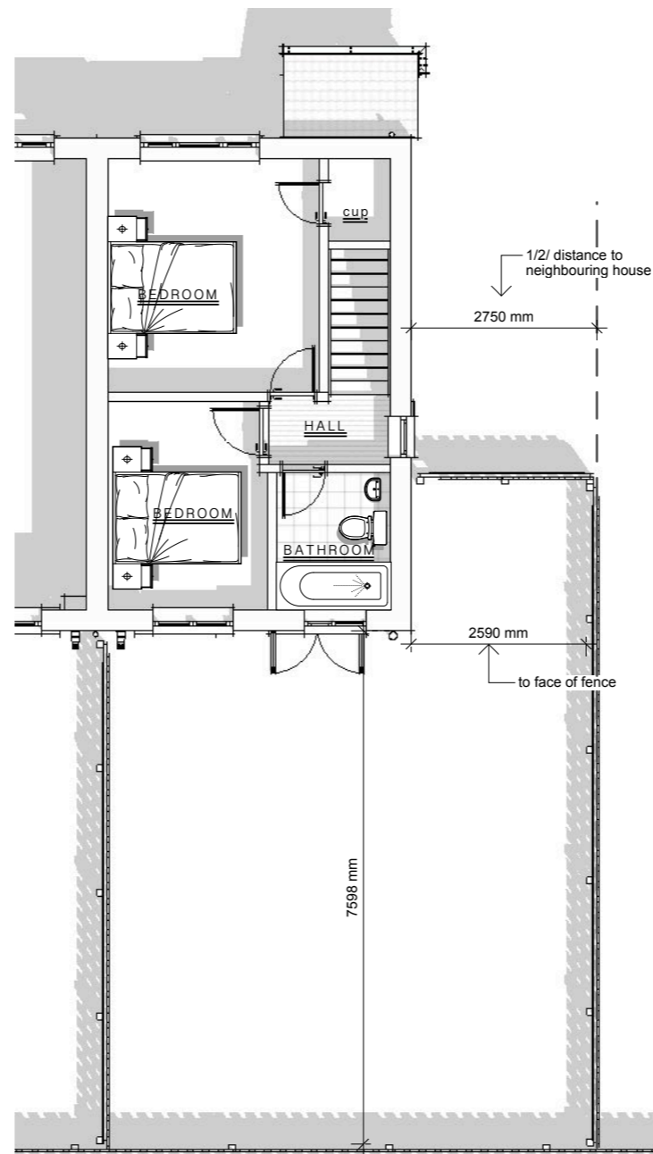
E 1 :: EXISTING FIRST FLOOR PLAN scale: 1:100
