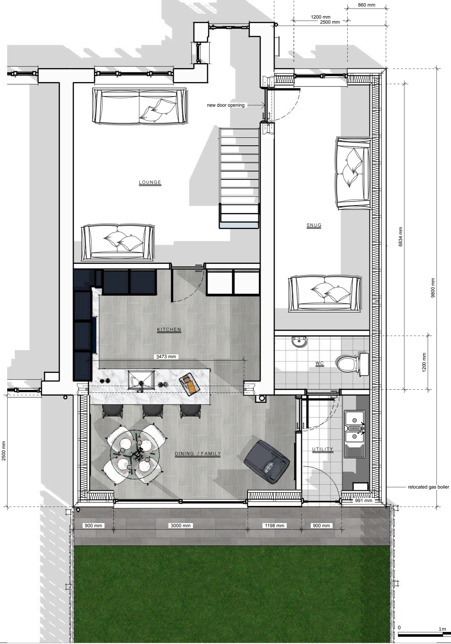
P :: PROPOSED GROUND FLOOR PLAN 2 scale: 1:50
