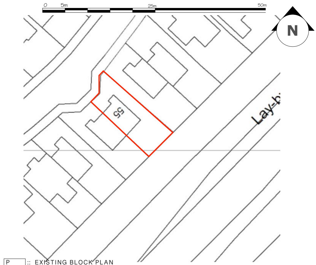
P :: EXISTING BLOCK PLAN 7 scale: 1:500
