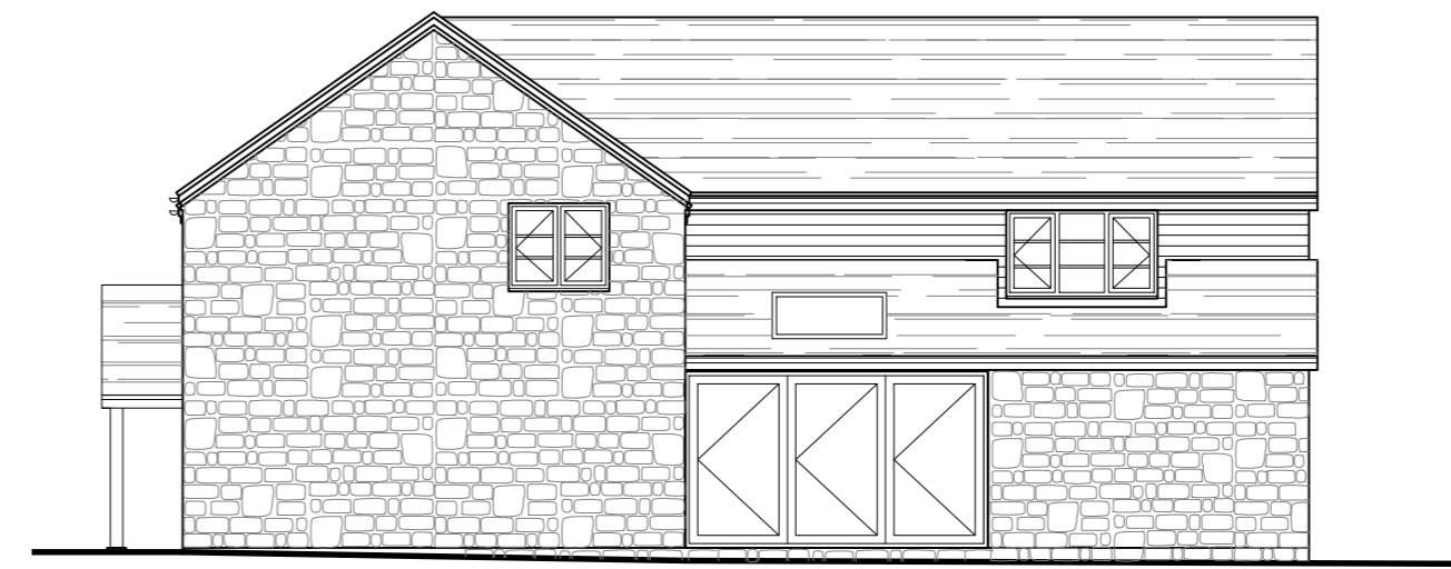
Side Elevation
