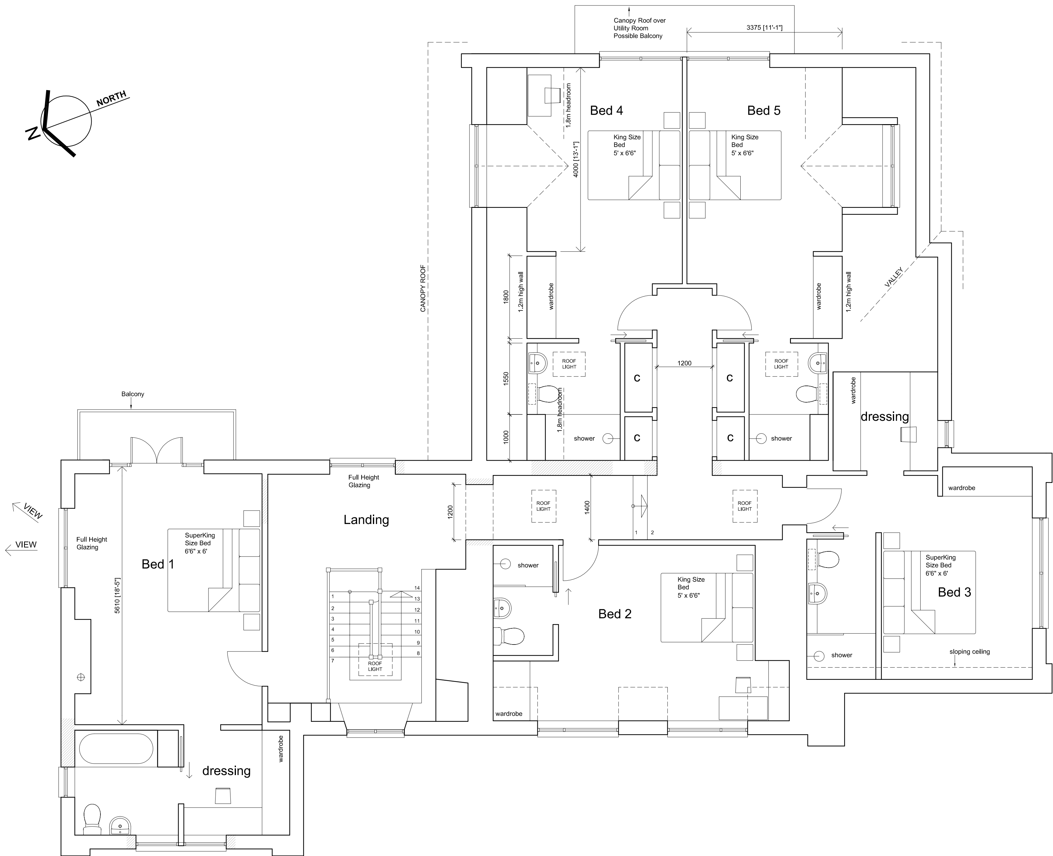
First Floor Plan As Proposed Scale 1:50
