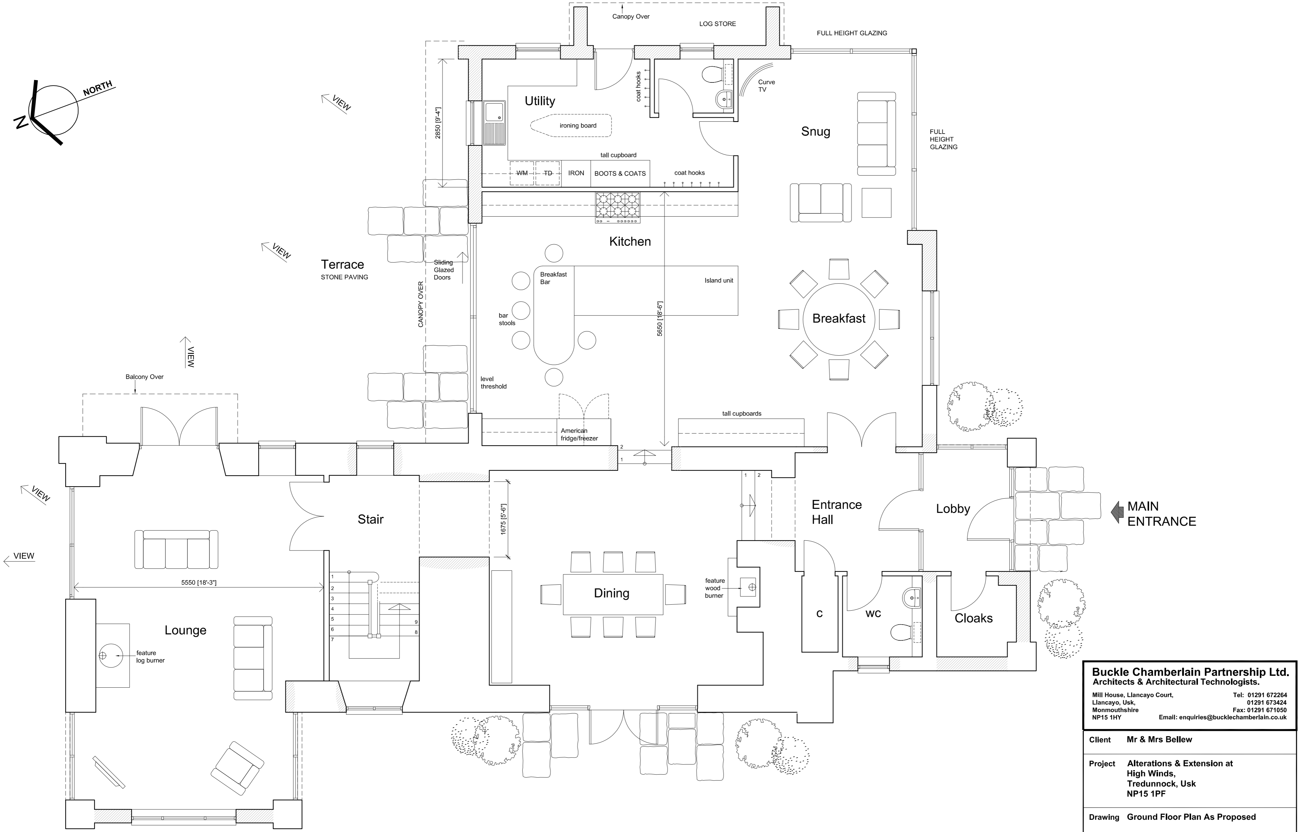
Ground Floor Plan As Proposed Scale 1:50
