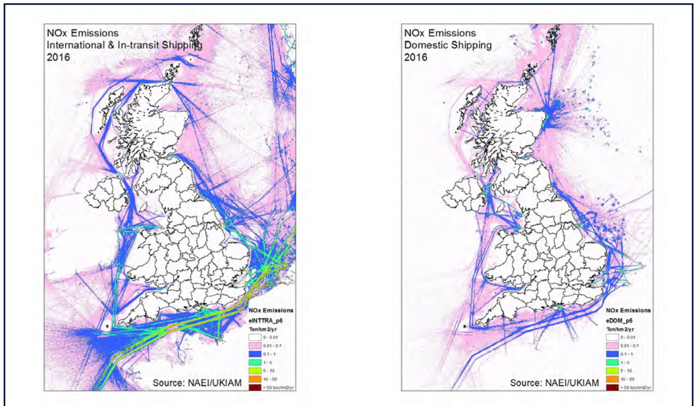
Figure 1: Shows the modelled contributions of NOx emissions from shipping and the geographical location of these emissions. This analysis was carried out by Imperial College based on AIS data.
