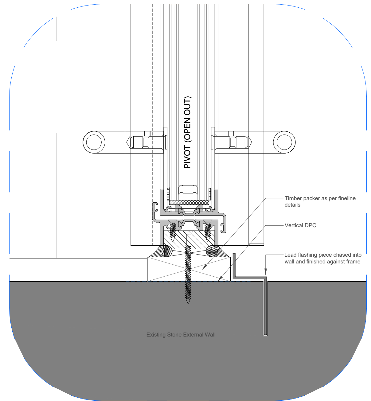
Detail 02 Flashing into existing fabric
