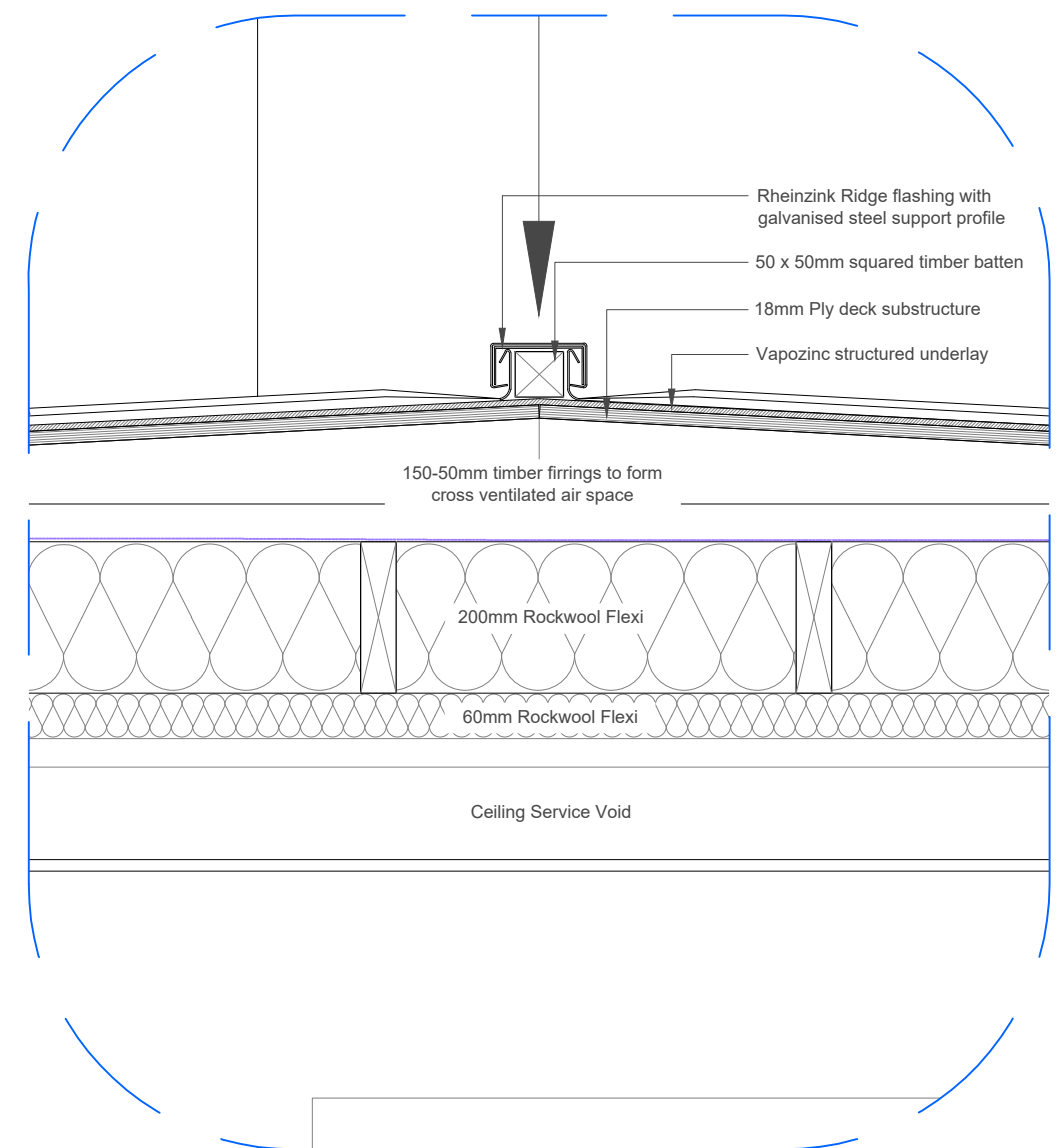
Detail 03 Ridge
