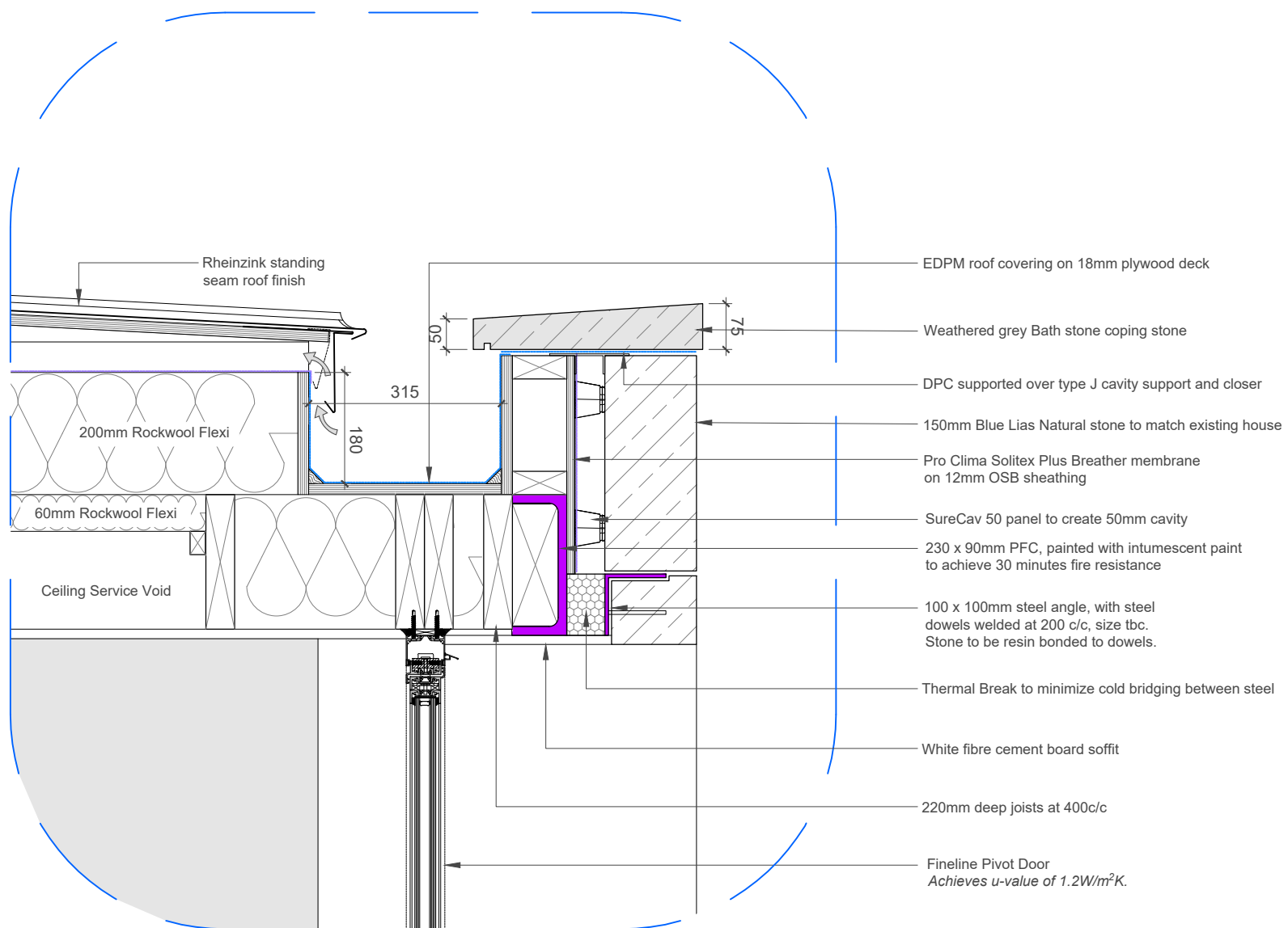
Detail 02 Eaves
