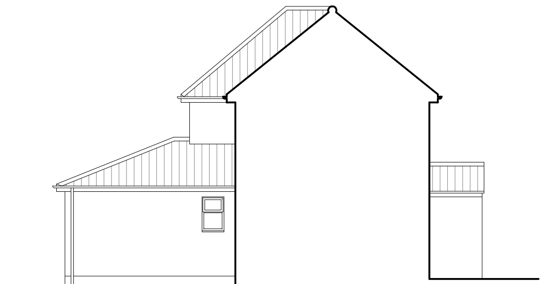
NORTH ELEVATION
