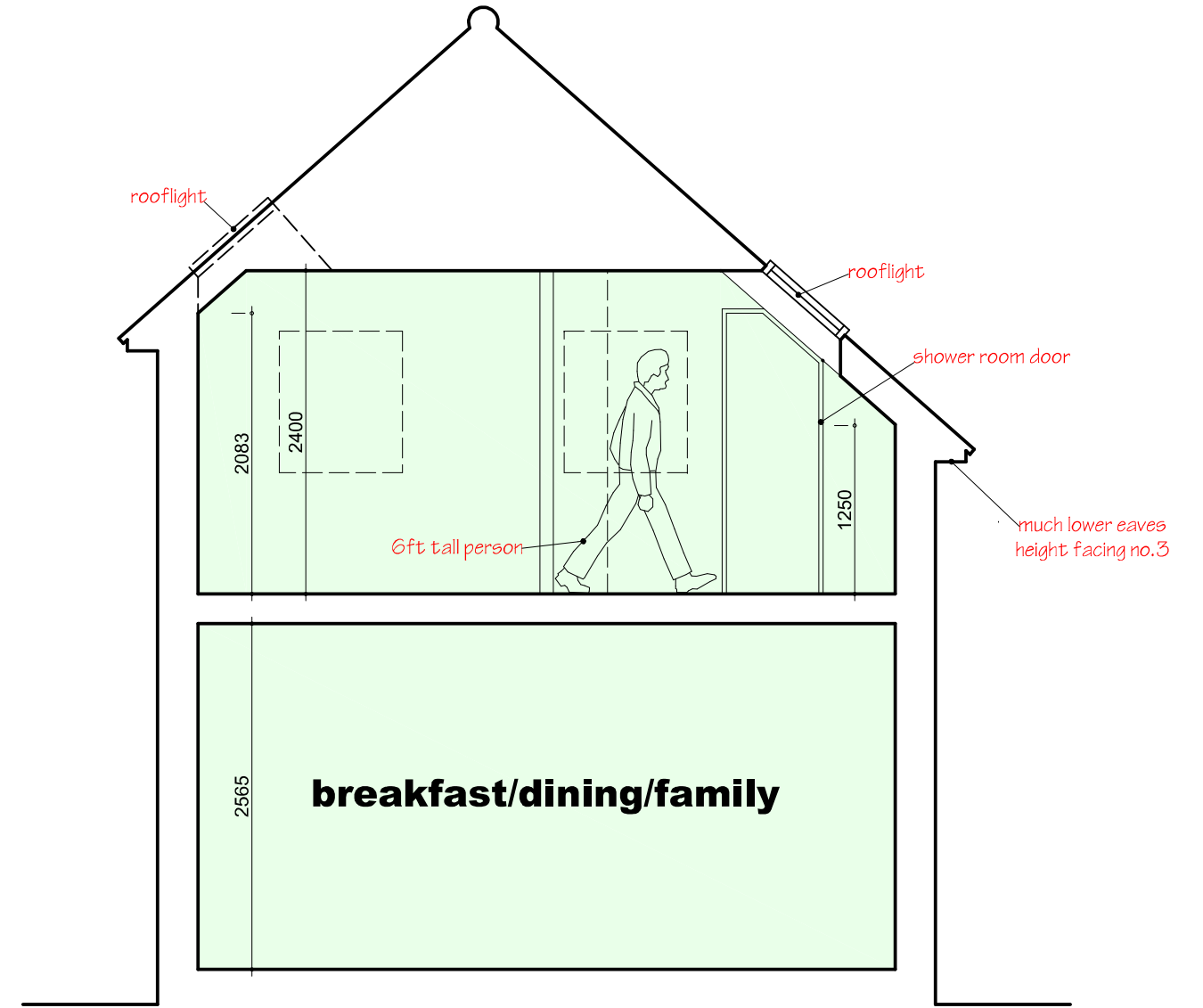
SECTION
