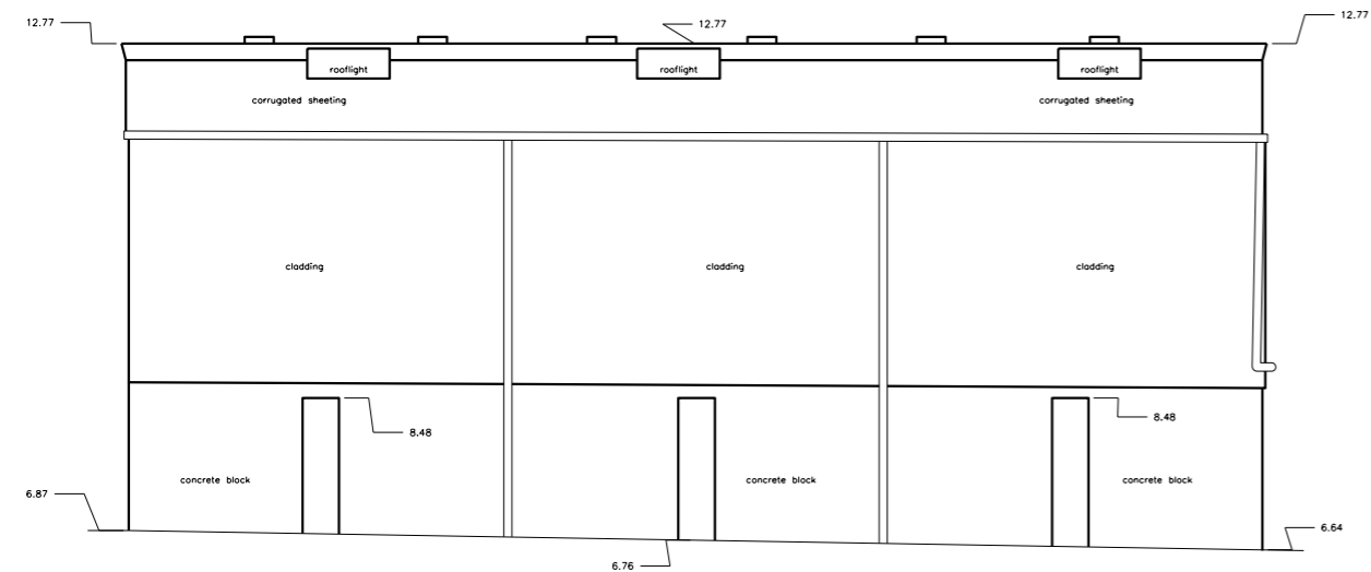
Existing: Northwest Elevation 1/100@A3
