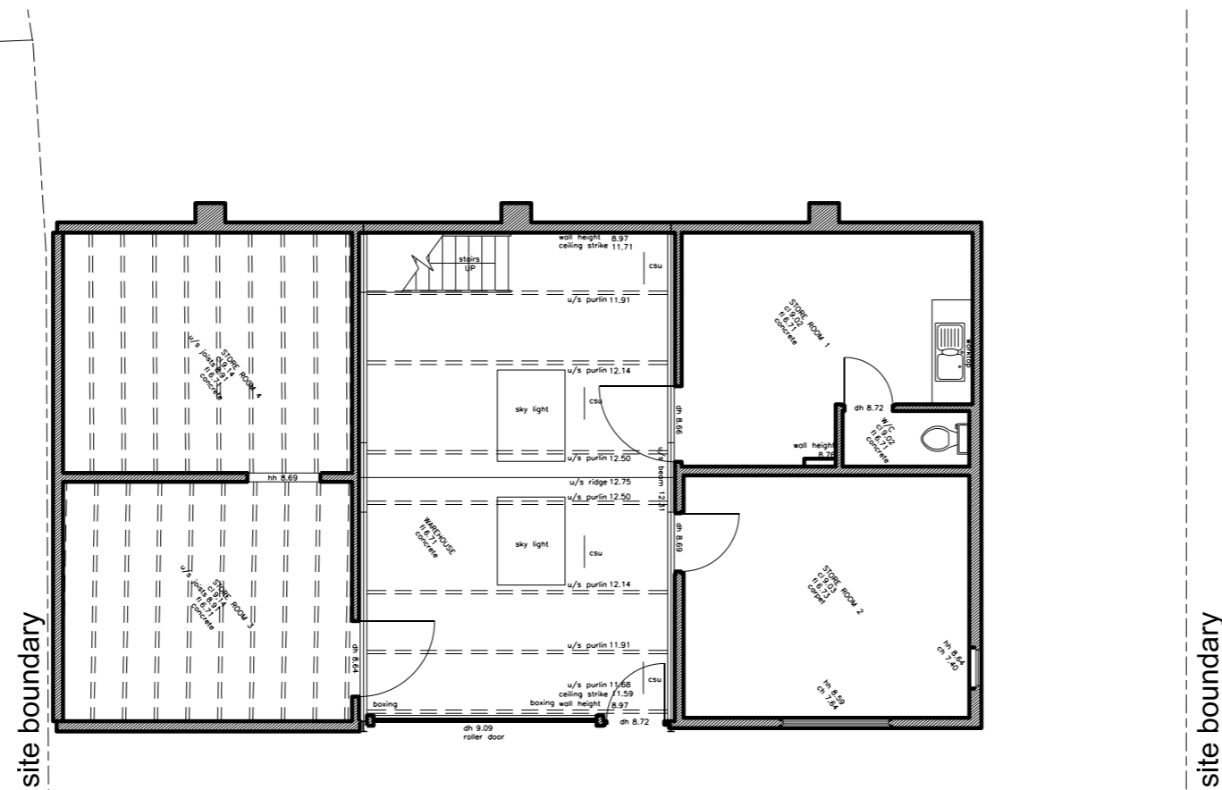
Existing: Ground Floor Plan 1/100@A3
