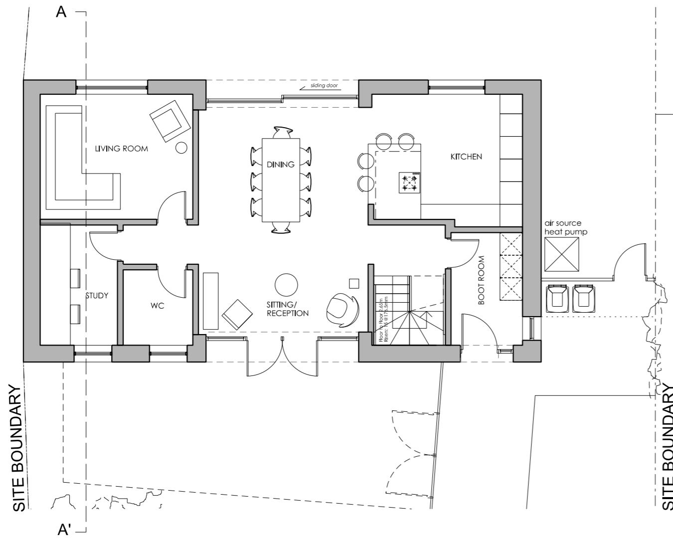
GROUND FLOOR PLAN 1:50 @A1
