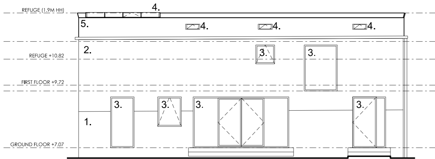
PROPOSED SOUTHEAST ELEVATION
