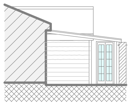
North Elevation
