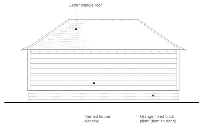
North Elevation
