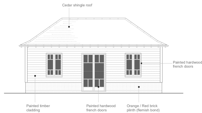
South Elevation
