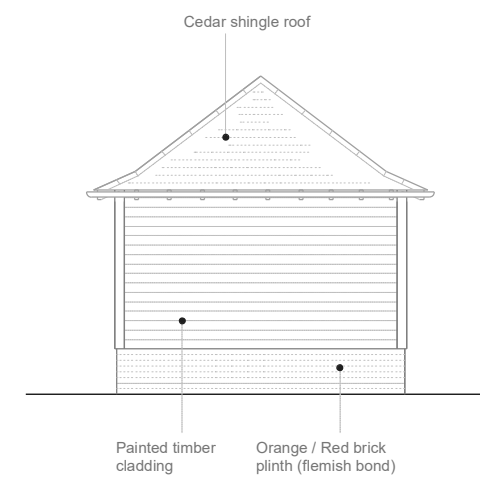
East Elevation
