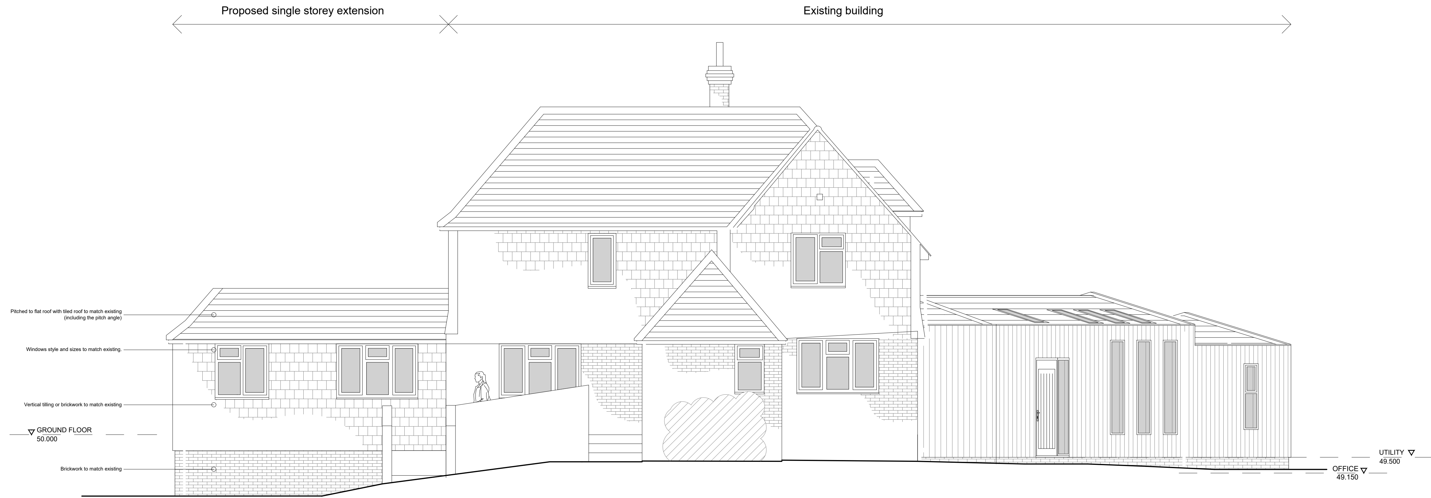
AS PROPOSED FRONT ELEVATION (E) 1:50 @ A1
