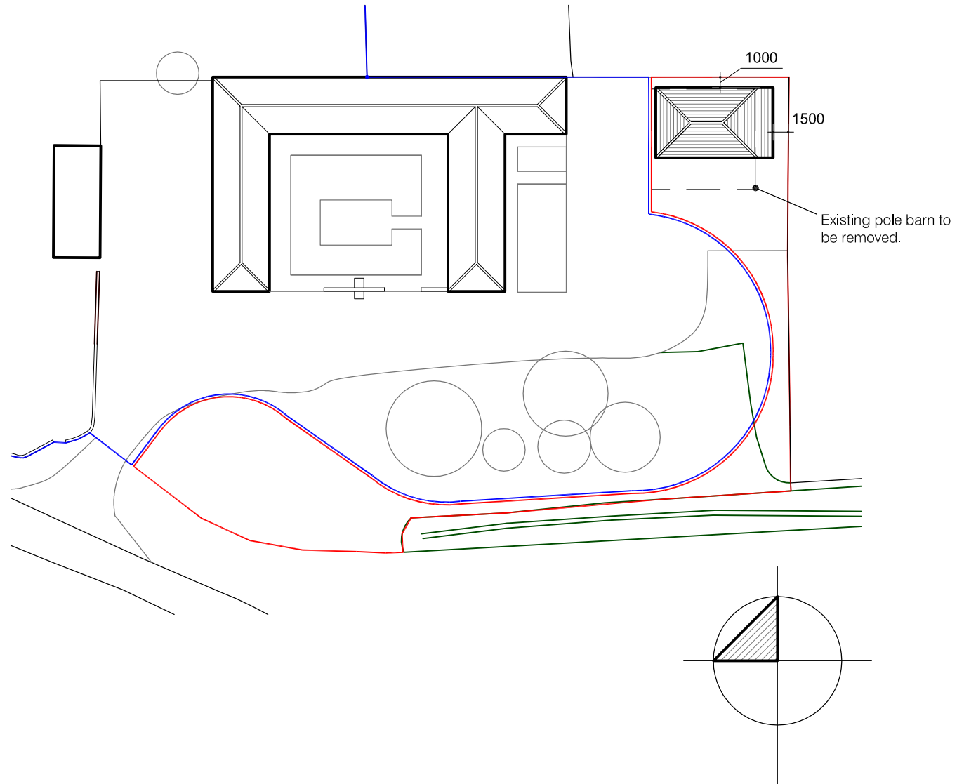
BLOCK PLAN 1:500
