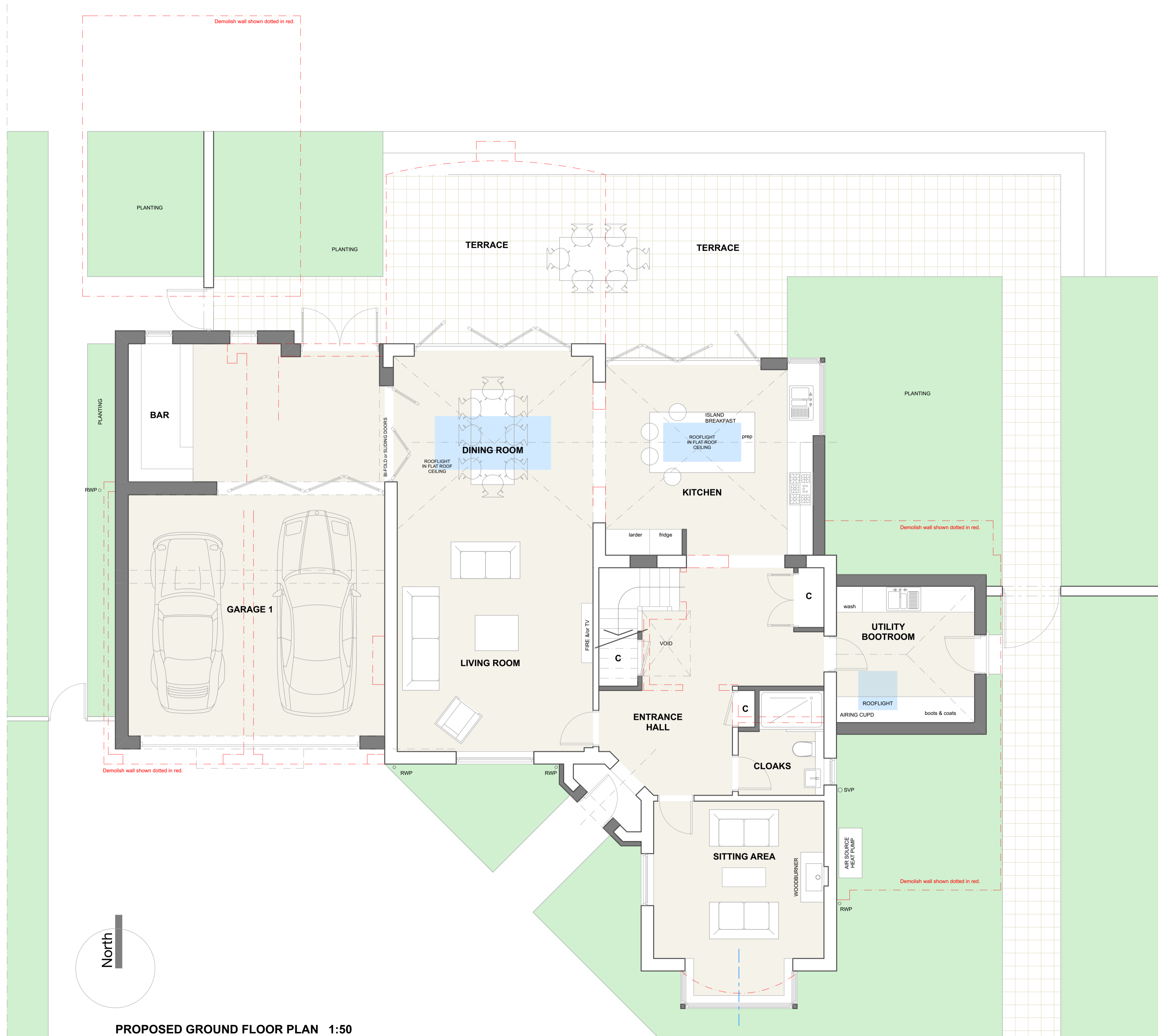
PROPOSED GROUND FLOOR PLAN 1:50
