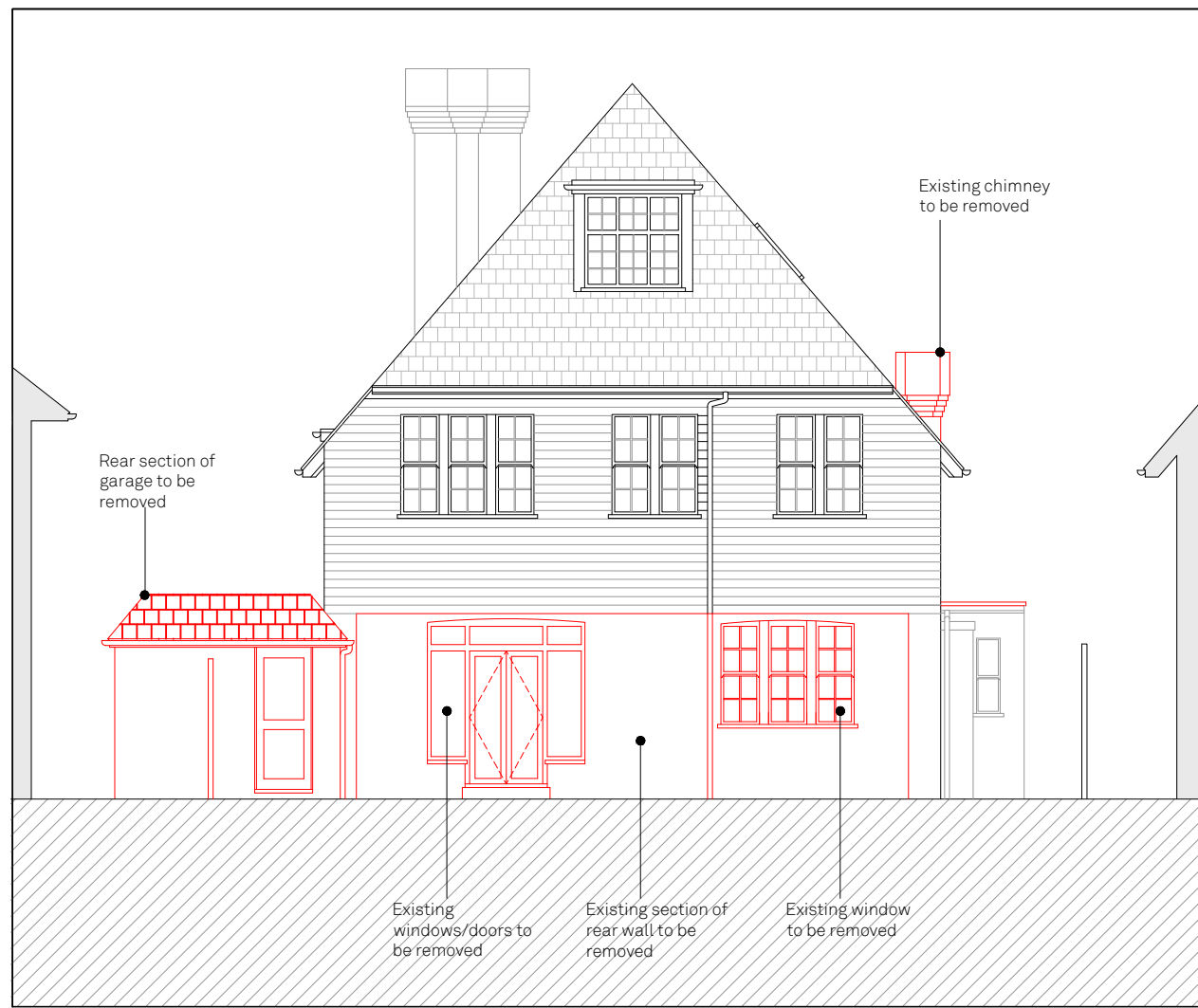
01 - EXISTING SHORT SECTION (DEMOLITION OUTLINED IN RED)
