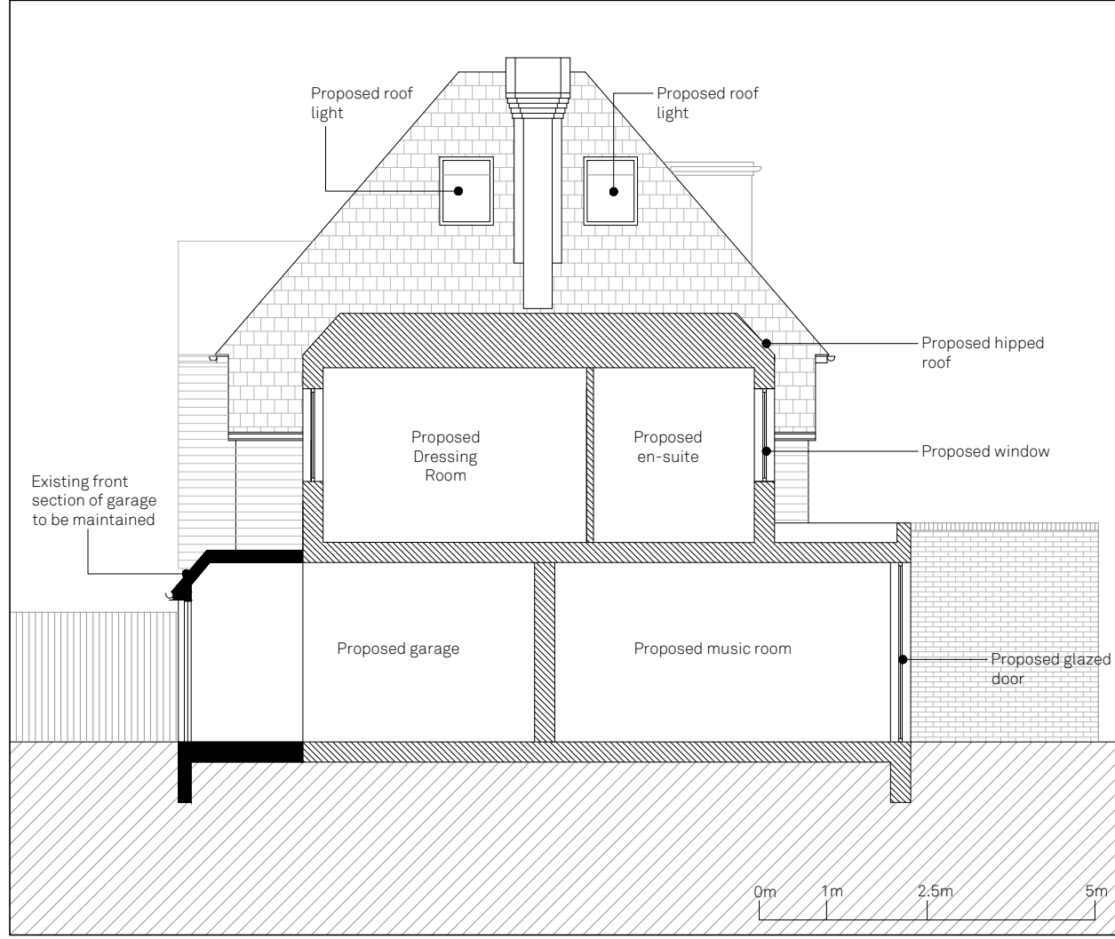
04 - PROPOSED LONG SECTION
