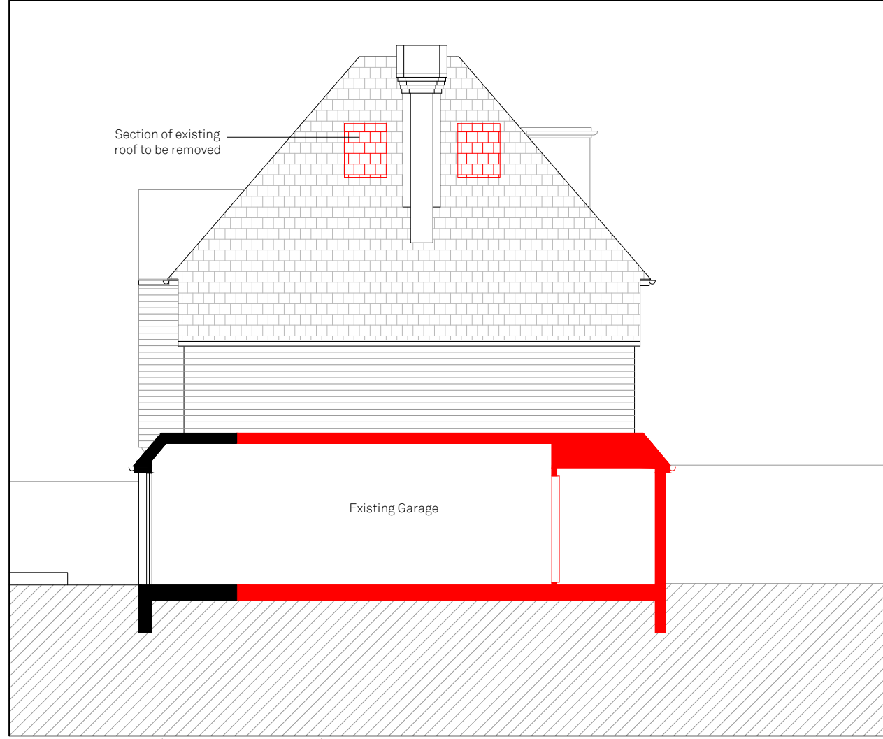
03 - EXISTING LONG SECTION (DEMOLITION OUTLINED IN RED)
