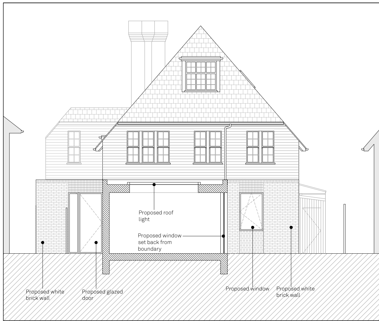
02 - PROPOSED SHORT SECTION
