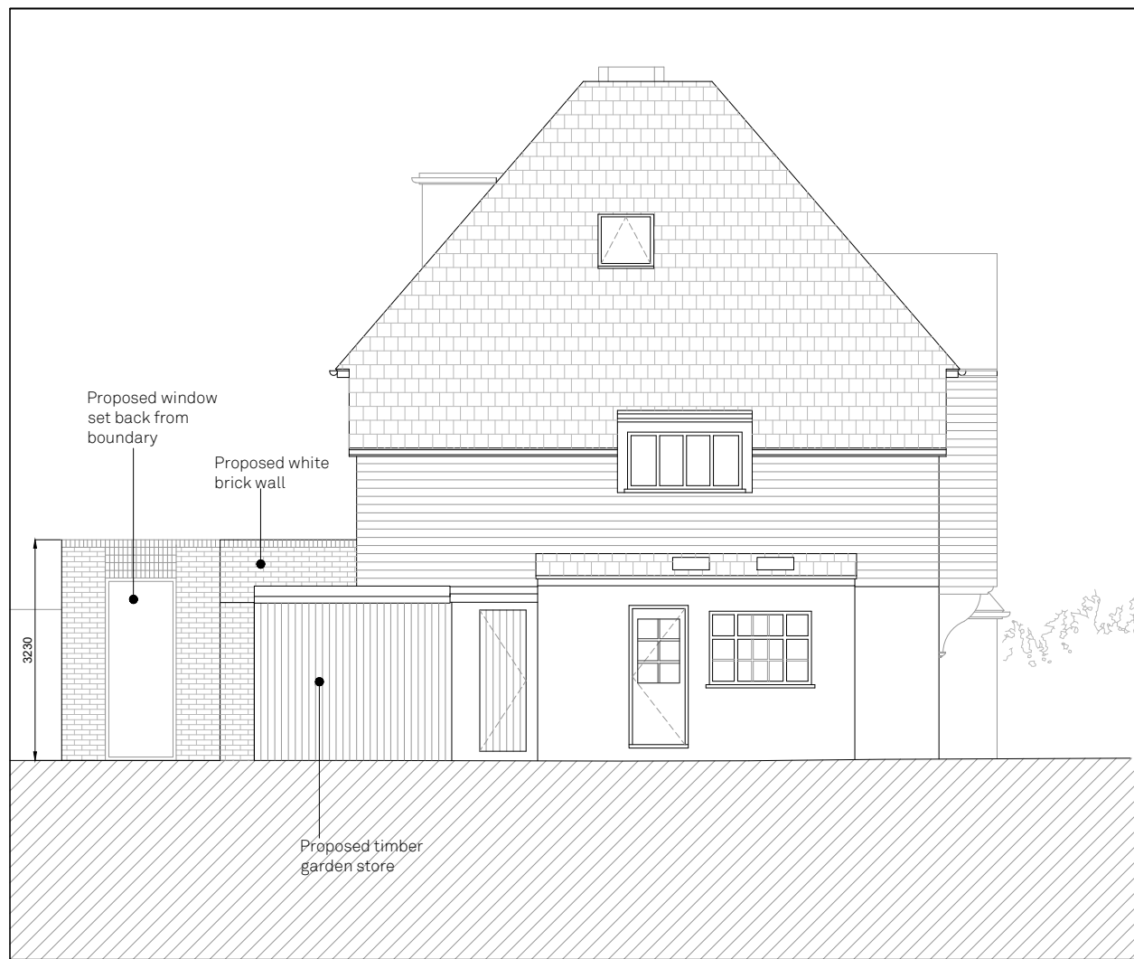
02 - PROPOSED EAST SIDE ELEVATION
