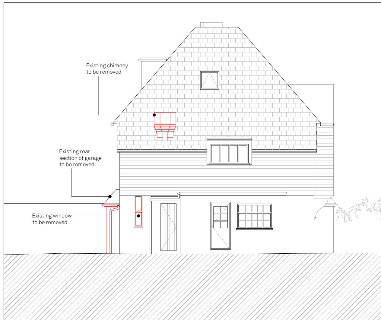
01 - EXISTING EAST SIDE ELEVATION (DEMOLITION OUTLINED IN RED)
