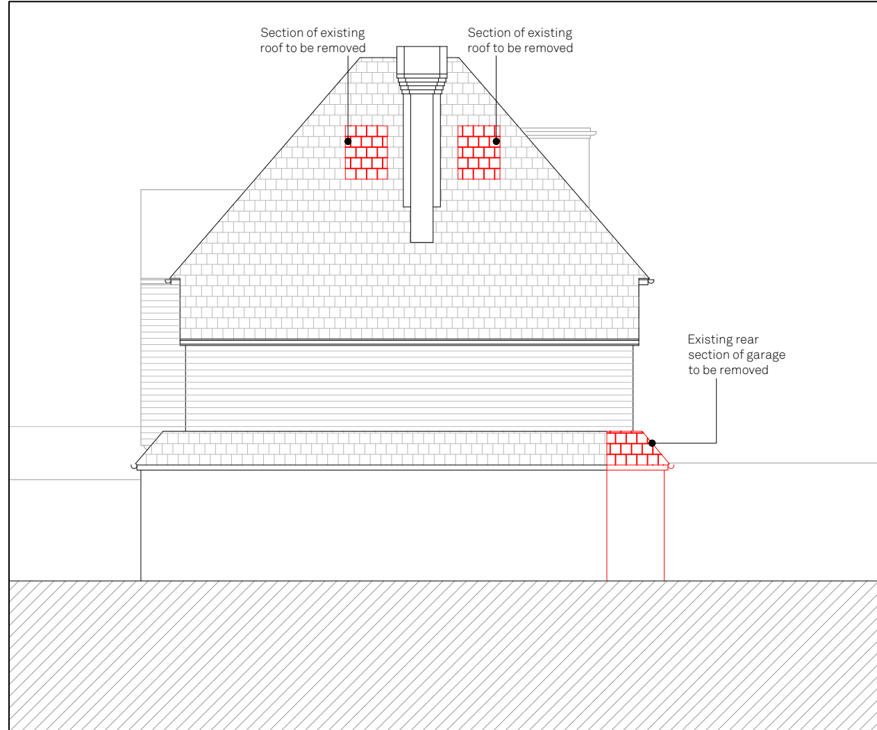
03 - EXISTING WEST SIDE ELEVATION (DEMOLITION OUTLINED IN RED)
