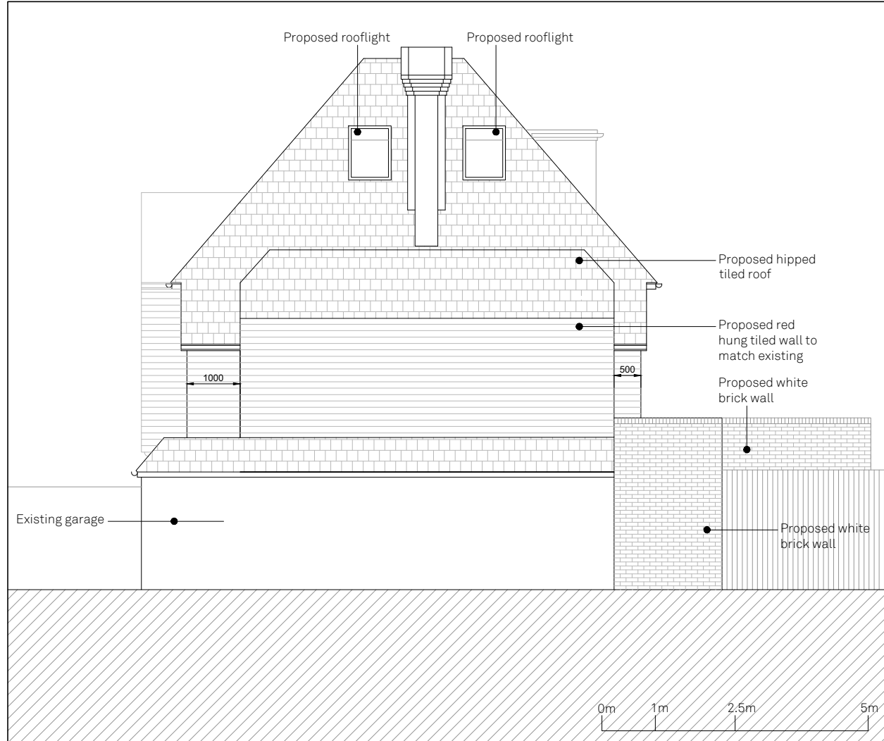
04 - PROPOSED WEST SIDE ELEVATION
