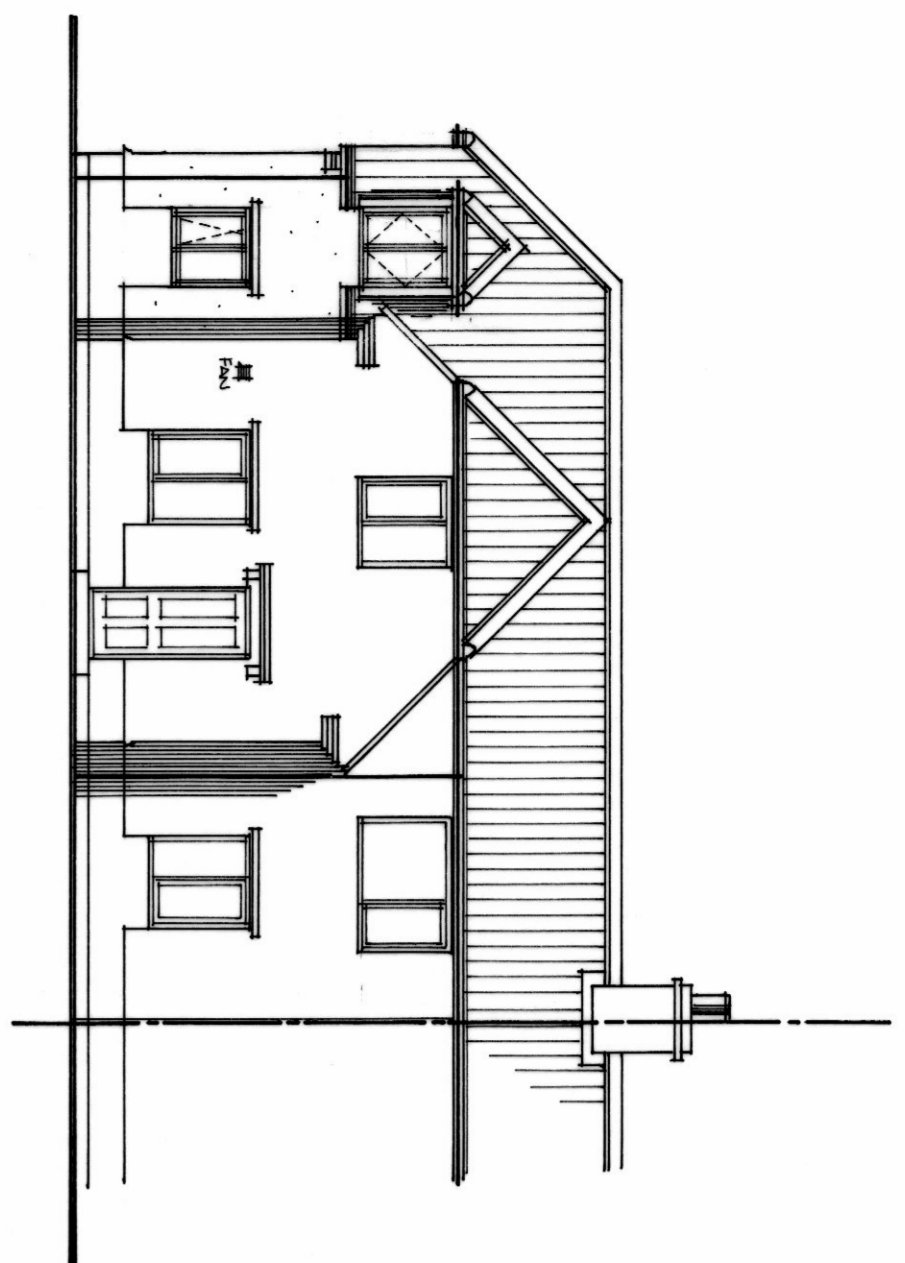
FRONT 1:100
