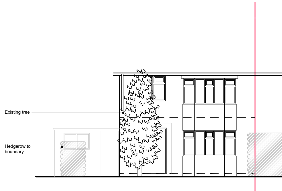
EXISTING SOUTHWEST (FRONT) ELEVATION 1:100
