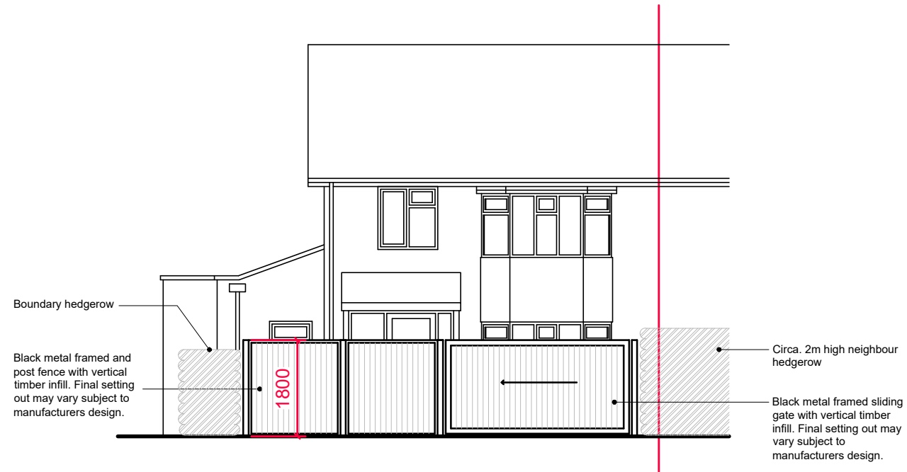
PROPOSED GATE (FRONT) ELEVATION 1:100
